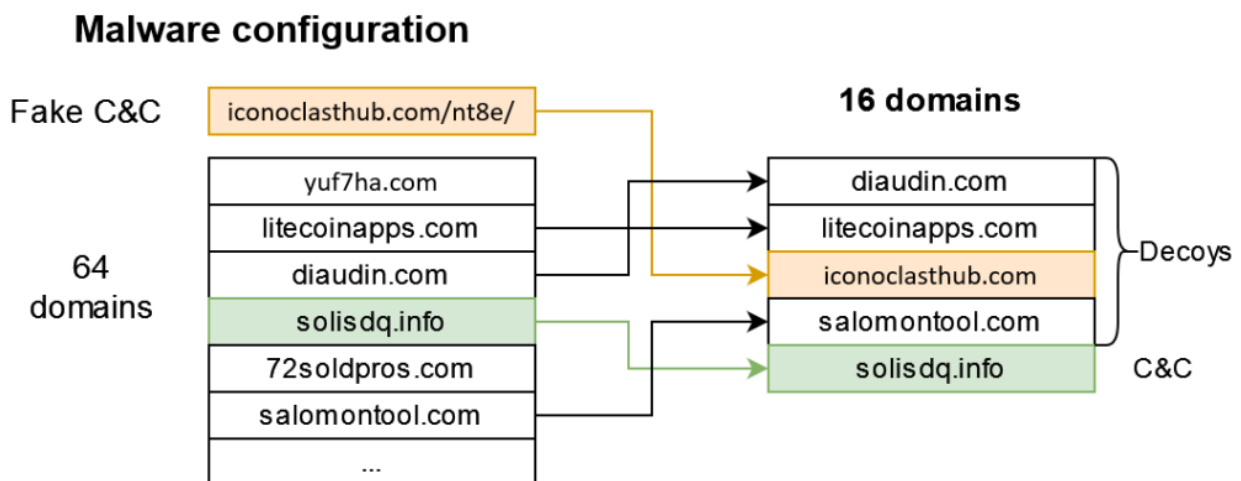
Figure 1 – Creating a list of domains for C&C communication in XLoader 2.3 and Formbook 4.1.
