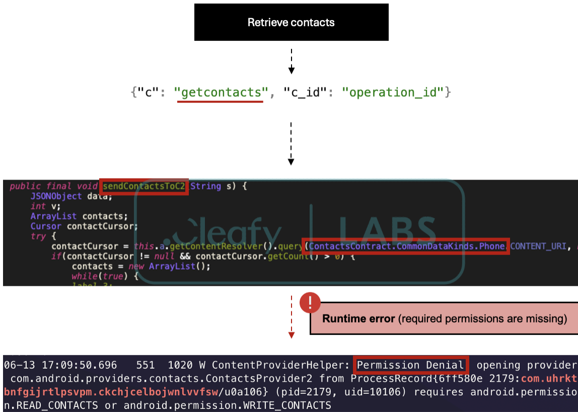
Figure 10 - Get Contacts Blocked
