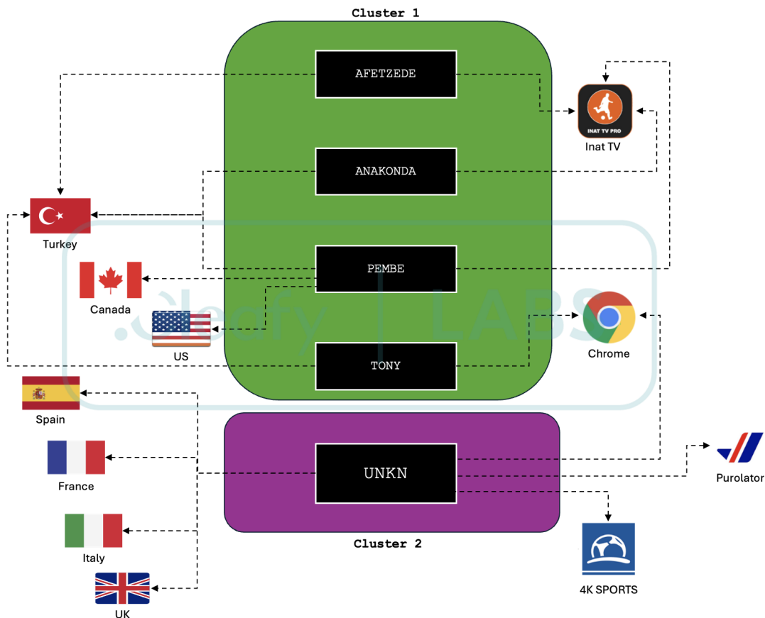
Figure 6 - Characteristics of the five botnets
