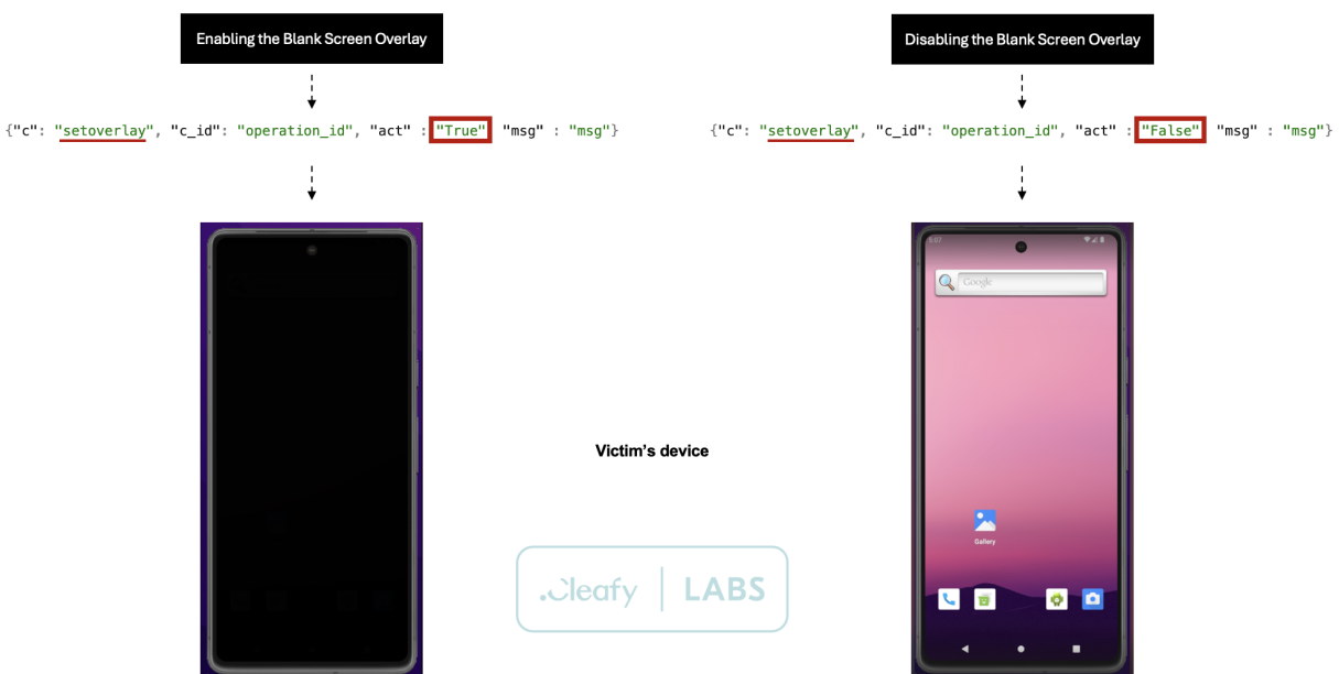
Figure 9 - Command “setoverlay” in action
