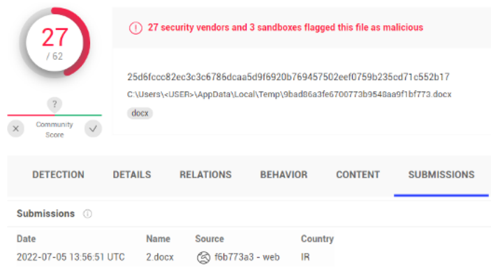
Figure 3: VirusTotal submission
