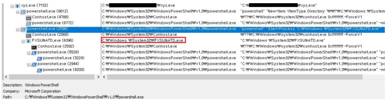
Figure 11. Process tree of Amadey downloader
