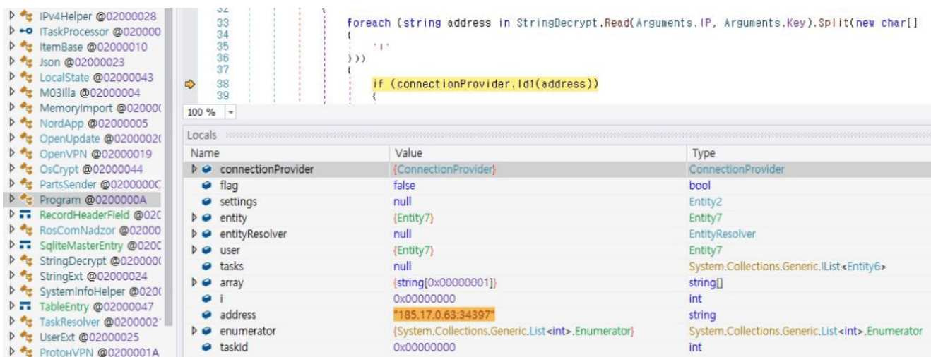
Figure 8. RedLine info-stealer being installed by Amadey Accessing “hxxp://185.17.0[.]52/” shows a list of files.
