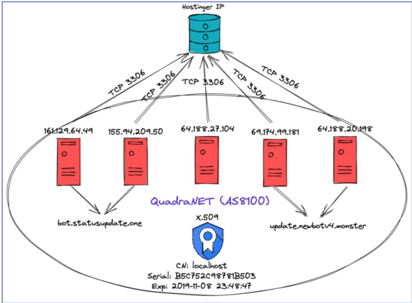
FIGURE 4: HOSTINGER MYSQL CLIENT RELATION
