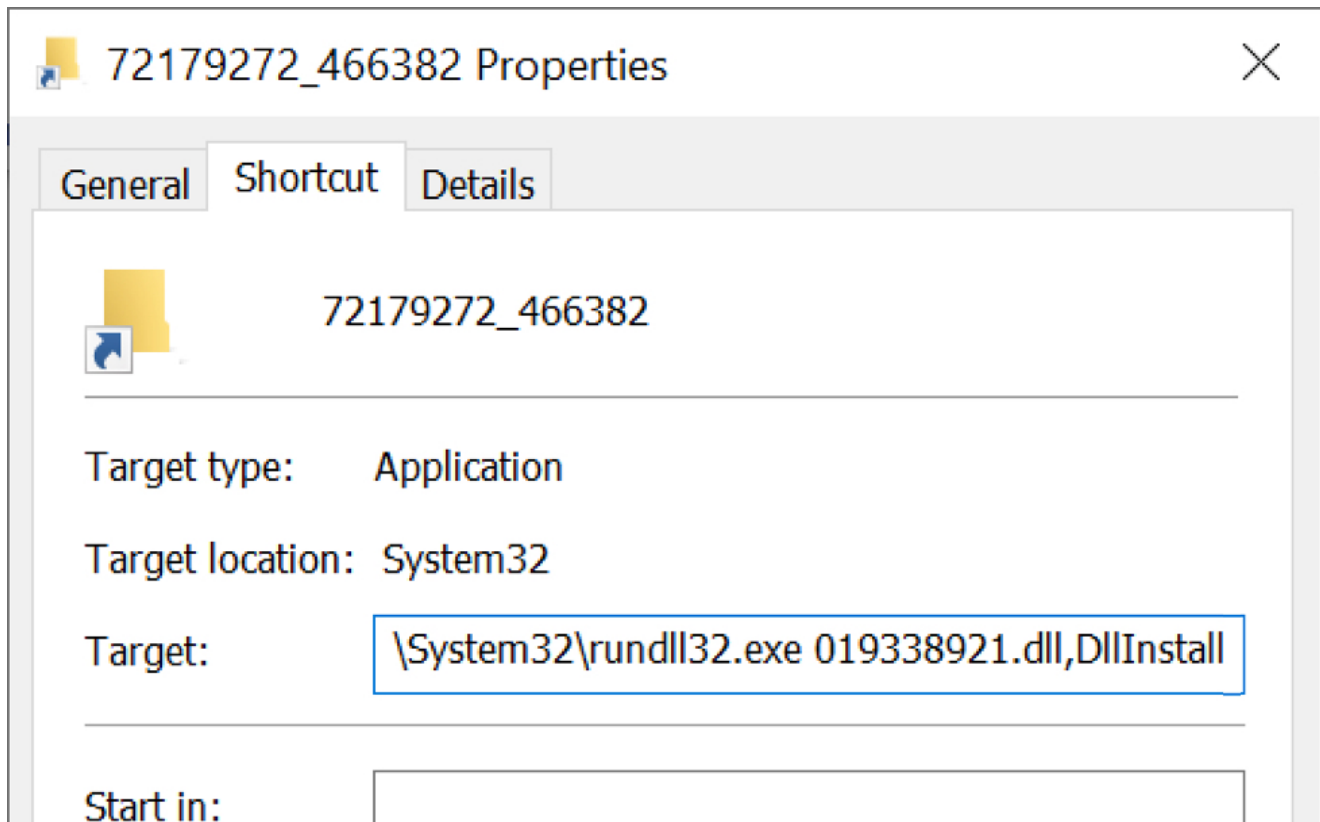
Shown above: Shortcut target uses rundll32.exe to run the hidden DLL file for Qakbot.
