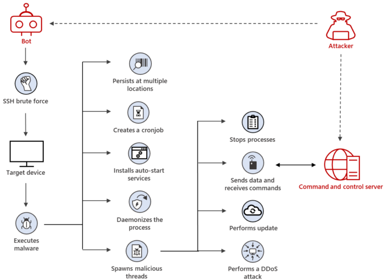
Figure 1. A typical attack vector for XorDdos malware
