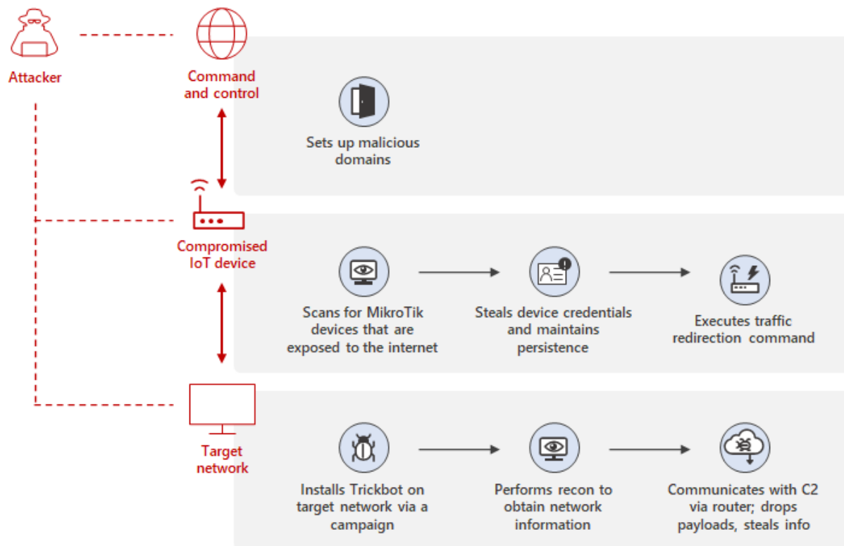
Figure 1. Trickbot attack diagram
