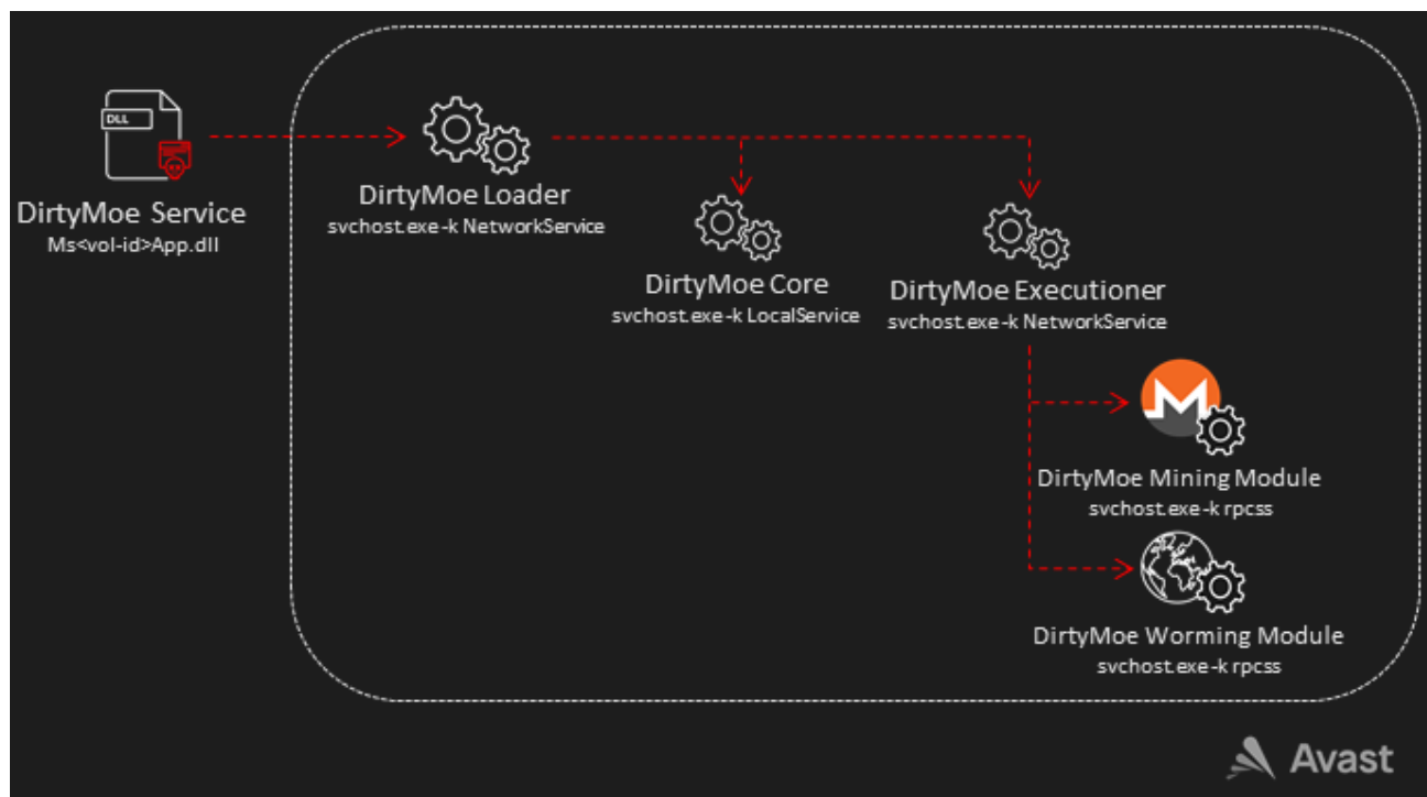
Figure 2. DirtyMoe hierarchy
