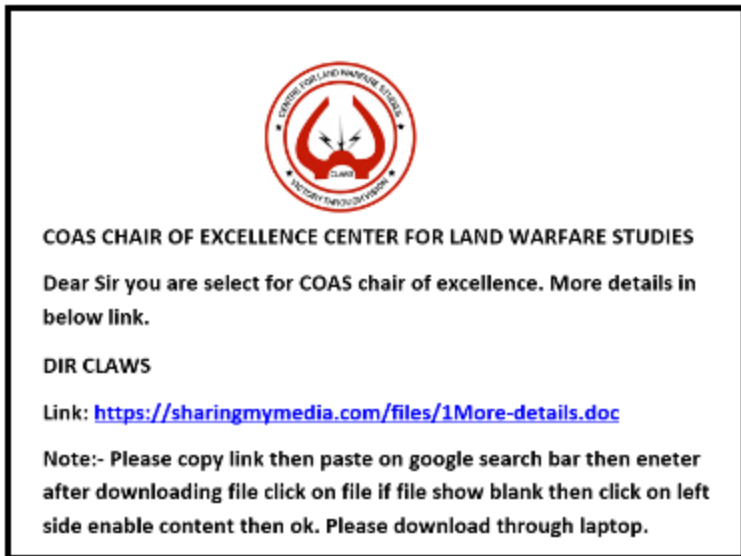
Figure 9. Initial spear-phishing
