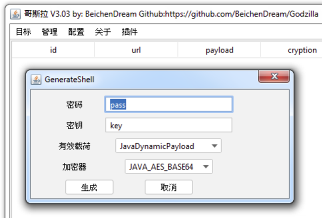
Figure 3. Godzilla default webshell values.
