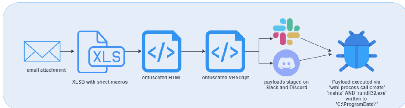
DoppelDridex infection chain
