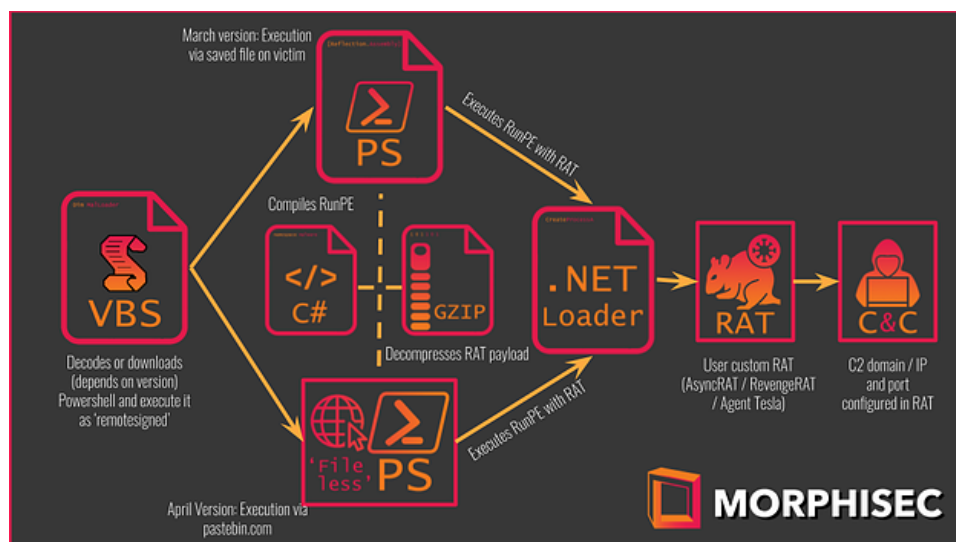
Figure 1 - The summarized execution flow
