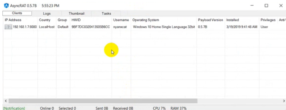
Figure 4 - AsyncRAT Panel
