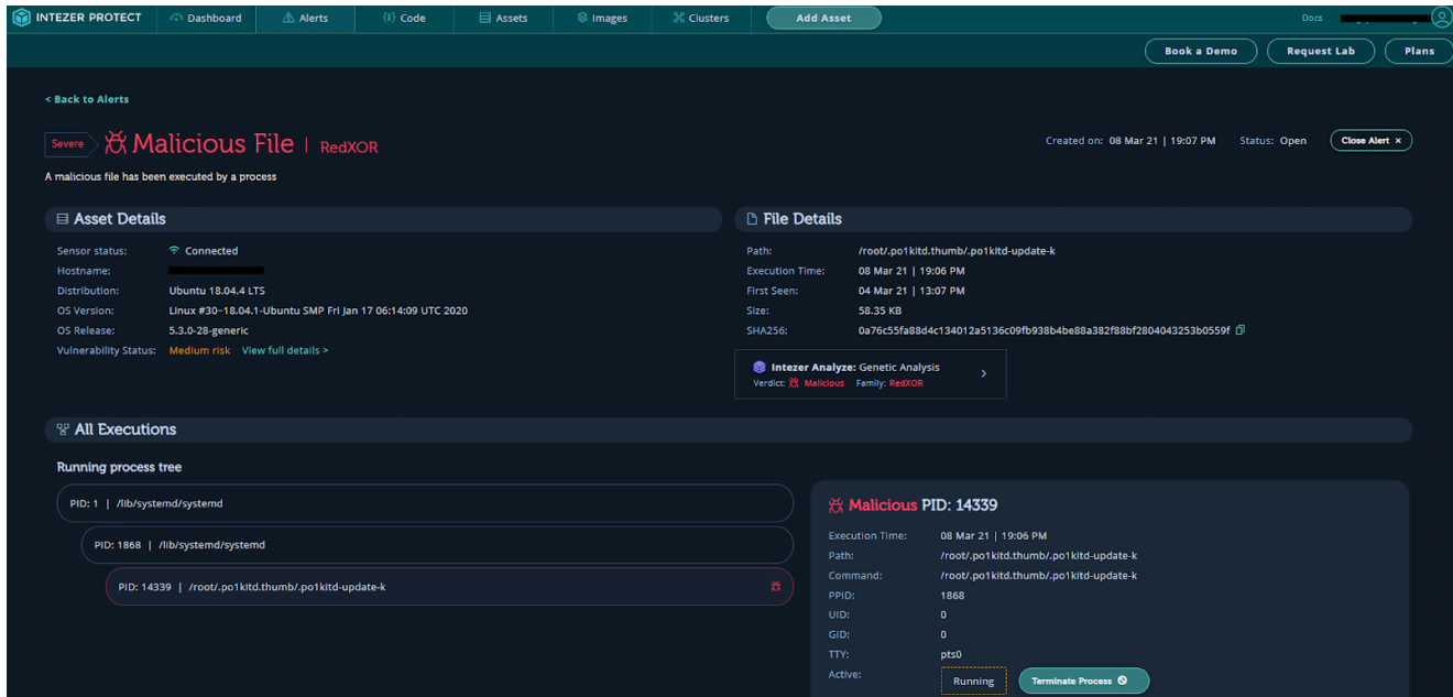
Figure 13: Intezer Protect alerts on RedXOR We also recommend using the IOCs section below to ensure that the RedXOR process and the files it creates do not exist on your system.
