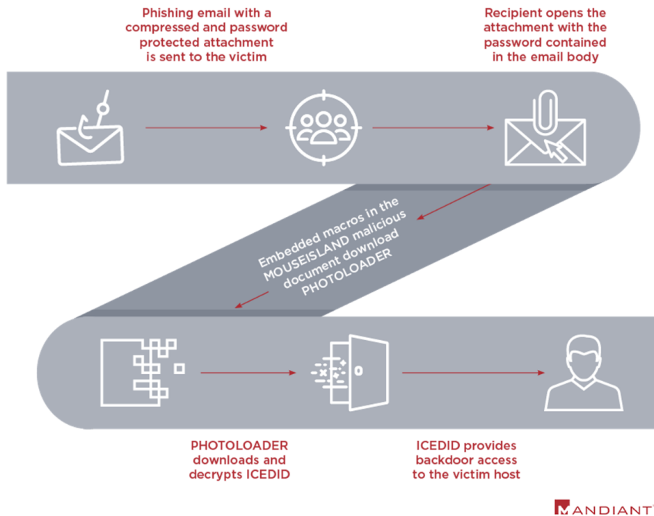
Figure 1: Example UNC2420 MOUSEISLAND to ICEDID Infection Chain
