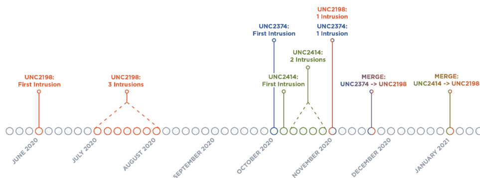
Figure 3: UNC2198 timeline
