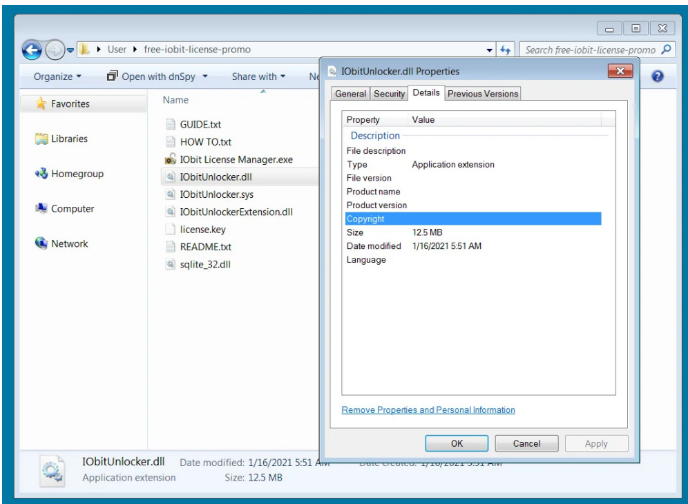
Malicious IObitUnlocker.dll
