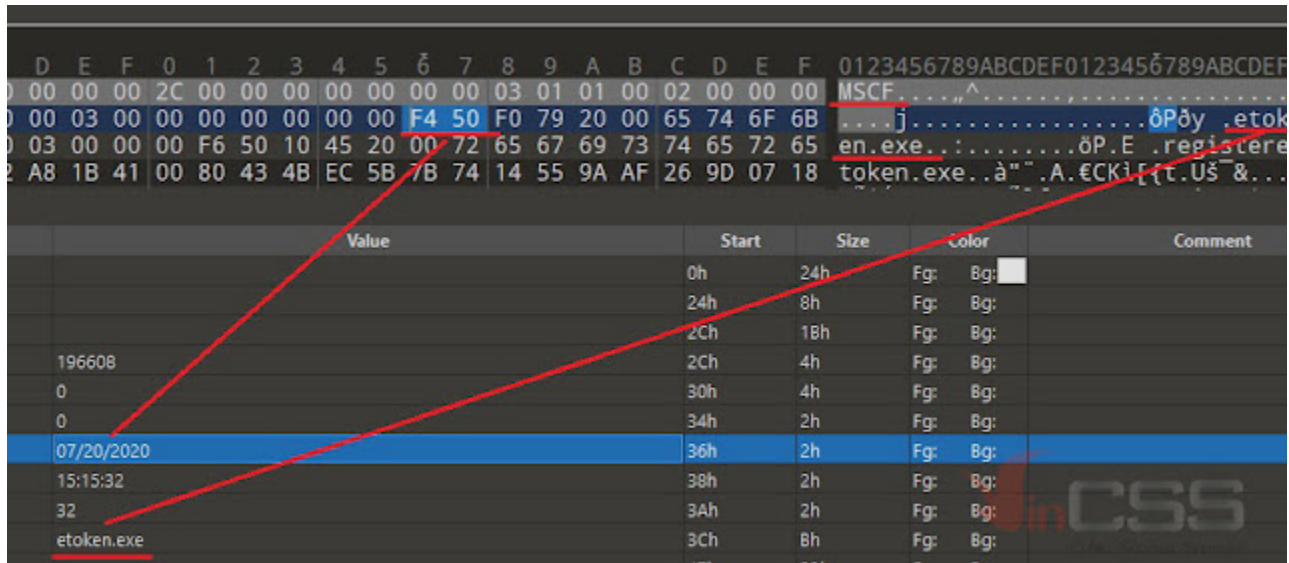
Figure 9. MS DOS Datetime Information
