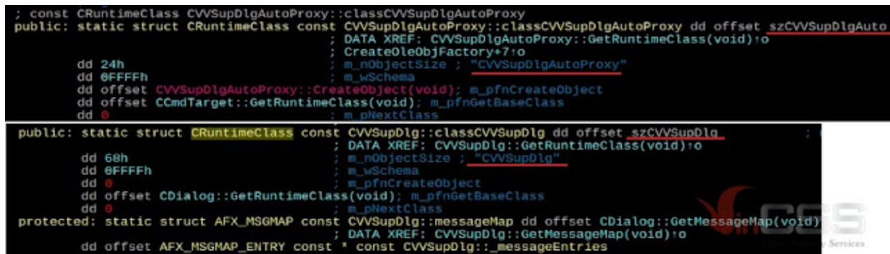
Figure 13. Detect classe after run MFC_Helper
