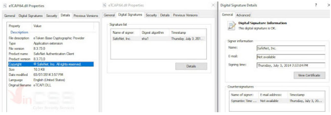
Figure 3. PE files signed with SafeNet certificate
