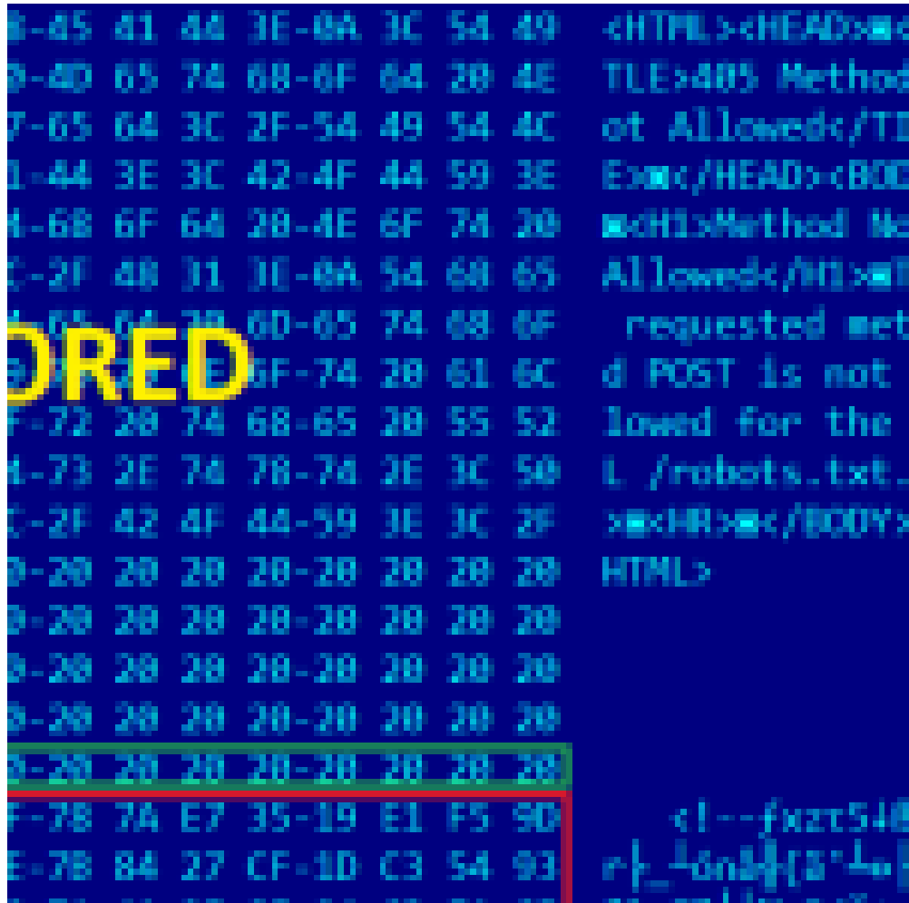
Figure 14. Example C&C server response including encrypted payload
