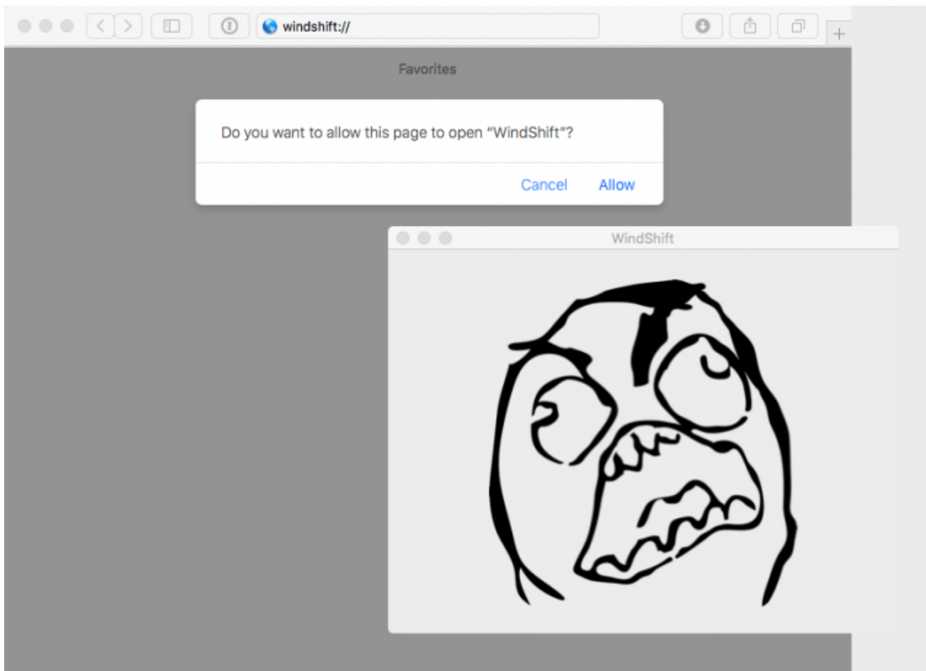
Figure 4: macOS launches the registered application.
