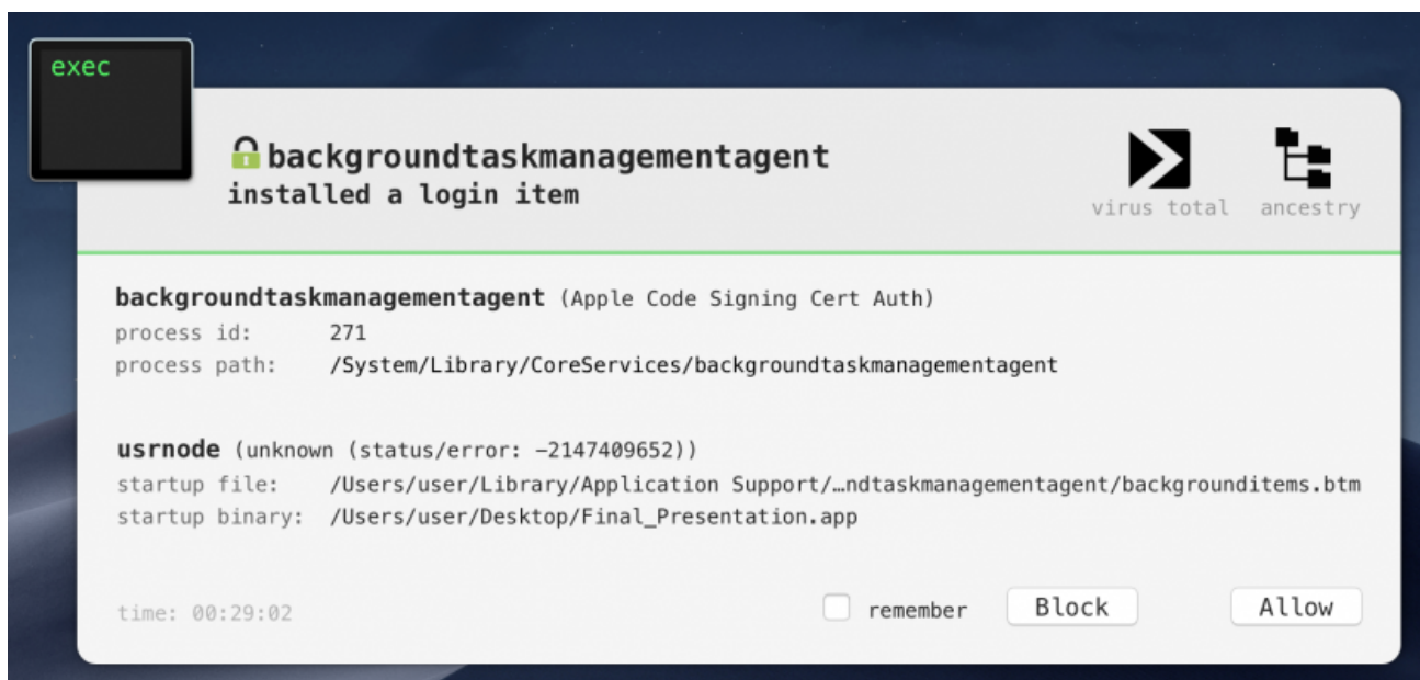
Figure 19: BlockBlock proactively detects OSX.WindTail.
