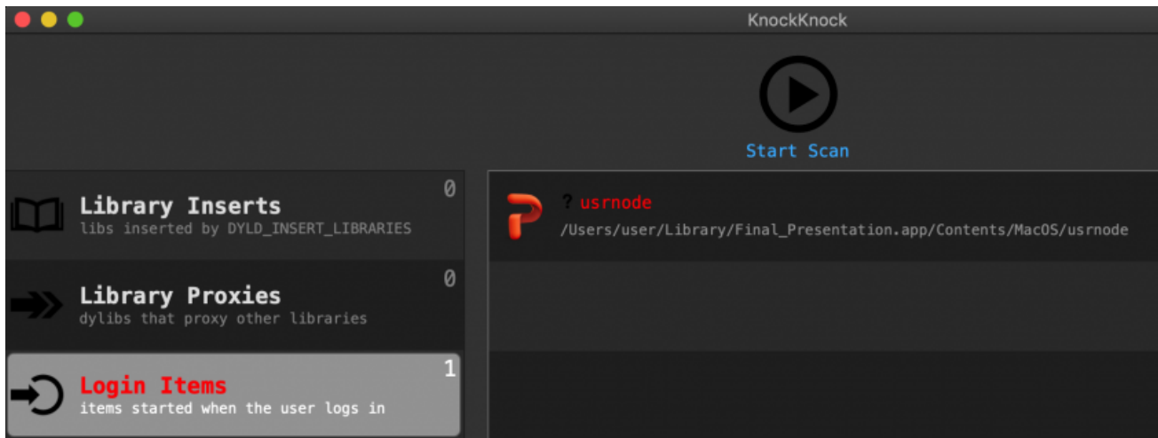
Figure 20: KnockKnock reactively detects OSX.WindTail.
