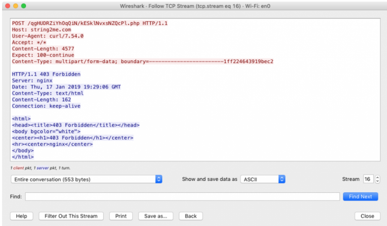
Figure 17: Exfiltration to string2me.com is attempted.
