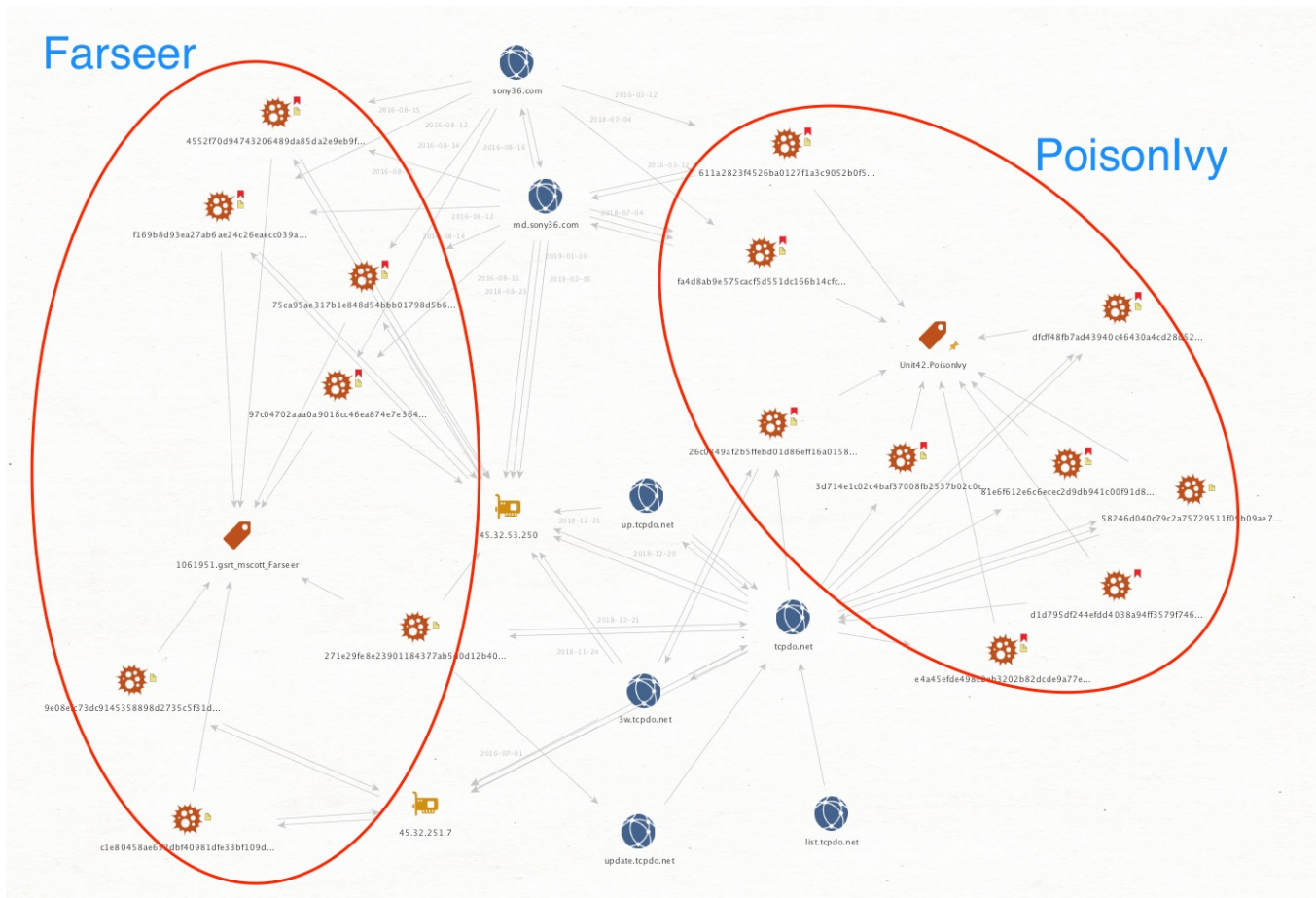
Figure 3 Maltego diagram showing tcpdo[.]net and other Farseer / PoisonIvy overlaps.
