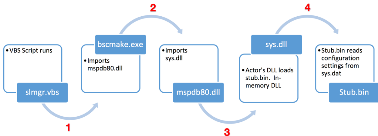
Figure 5 Farseer Execution Flow
