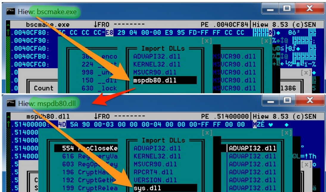
Figure 6 bscmake.exe importing mspdb80.dll importing Farseer's sys.dll
