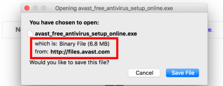
Figure 12: The Avast website in February 2018, showing an HTTPS padlock while automatically starting an insecure file download. The lack of HTTPS on the file download means that targeted users in Turkey and Syria will instead receive spyware. Avast fixed this particular issue in late February 2018.
