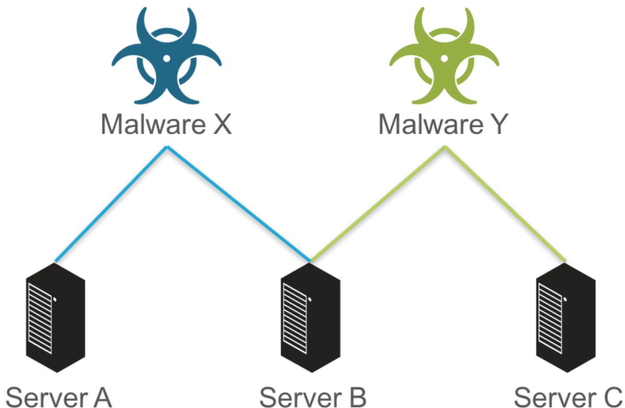
Figure 6 Malware redundancy
