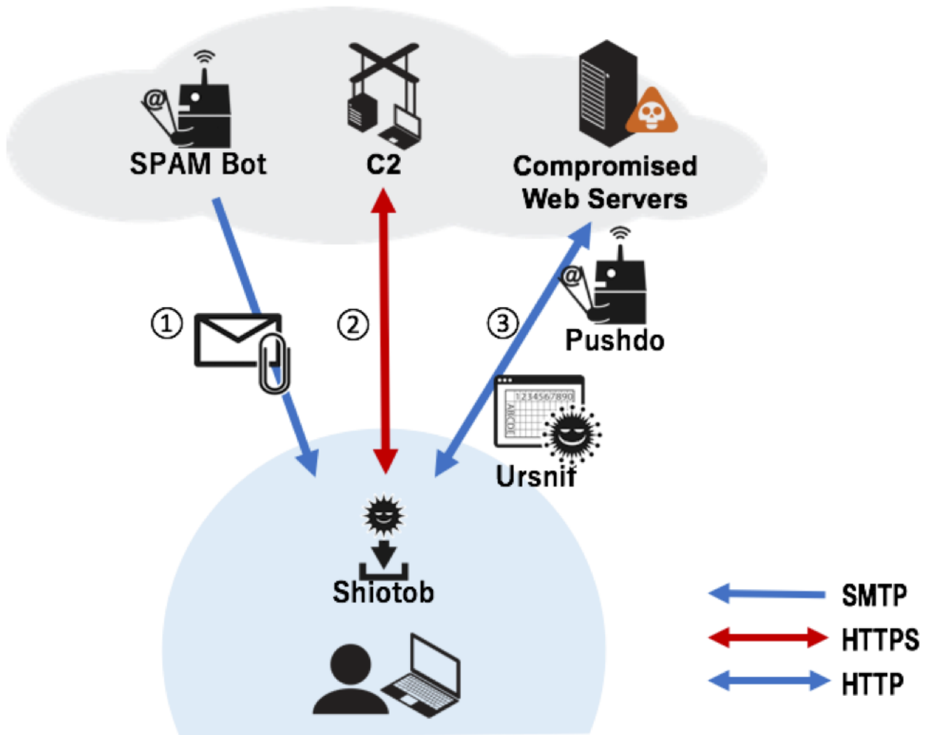
Figure 2 Infection steps
