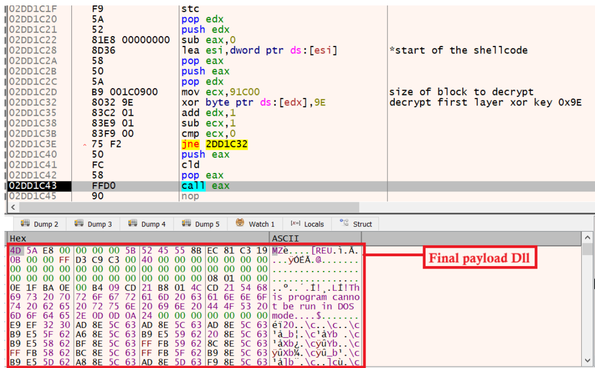
Figure(6) Shellcode transfers execution to final payload DLL export
