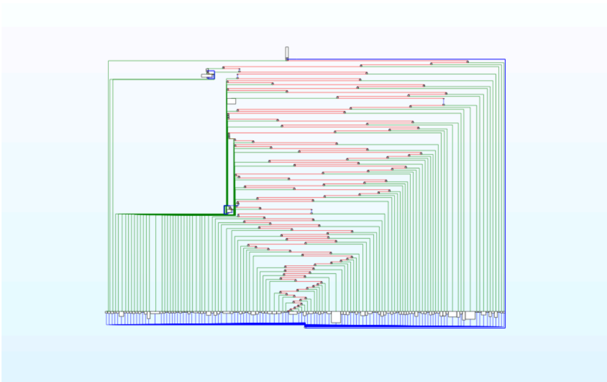
Figure(8) Control Flow Flattening Obfuscation
