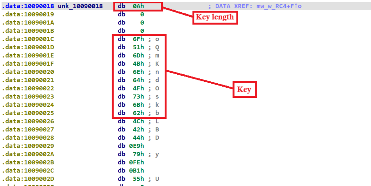
Figure(9) The configuration blob for RC4 The structure of the encrypted configuration information is :
