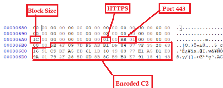
Figure(10) Configuration information for the decrypted PlugX variant
