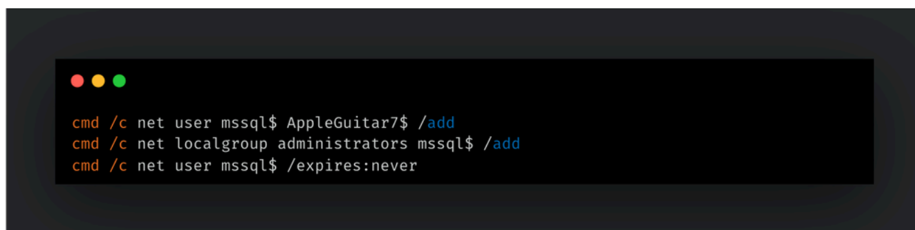
Figure 2. New user account named “mysql$”.
