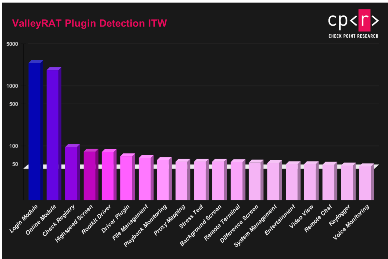
Figure 9: Statistics – ValleyRAT plugin detection (ITW).
