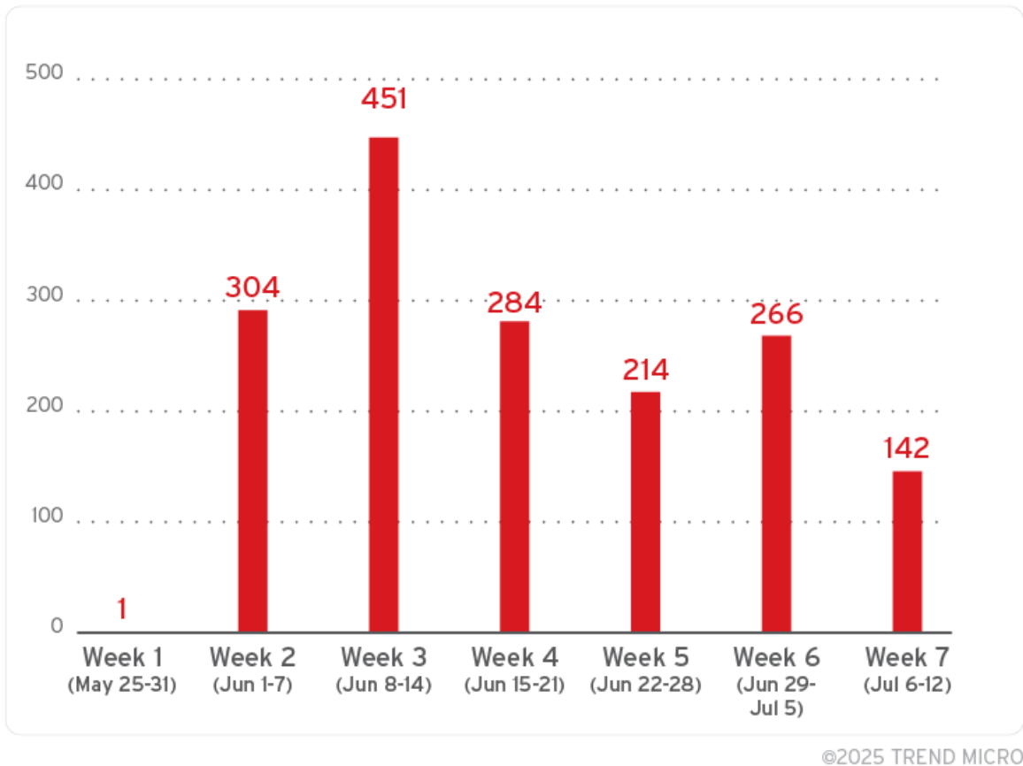
Figure 2. Hunted Lumma C&C URLs from Trend Micro telemetry download
