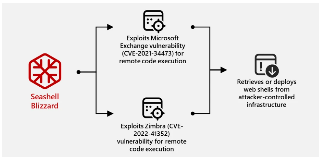
Figure 5. Seashell Blizzard exploitation of CVE-2021-34473 and CVE-2022-41352
