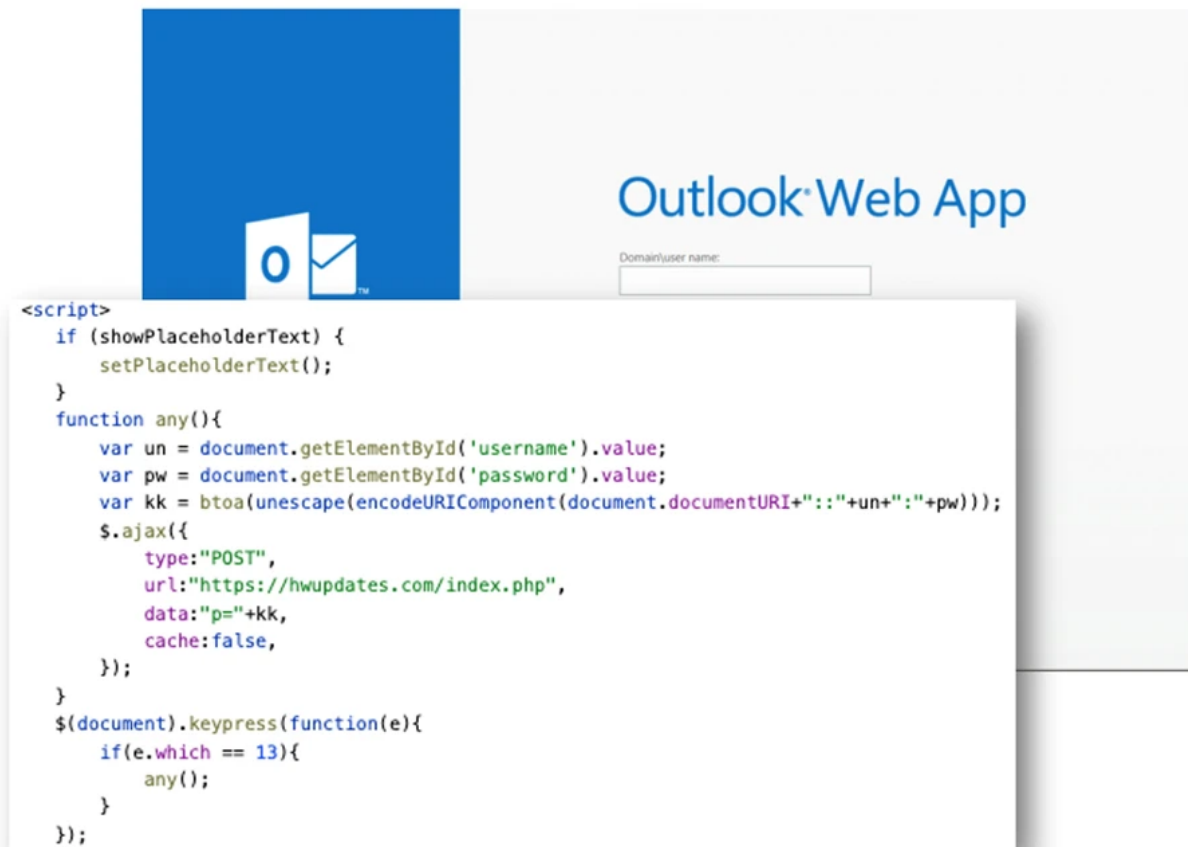
Figure 9. Seashell Blizzard credential collection from OWA
