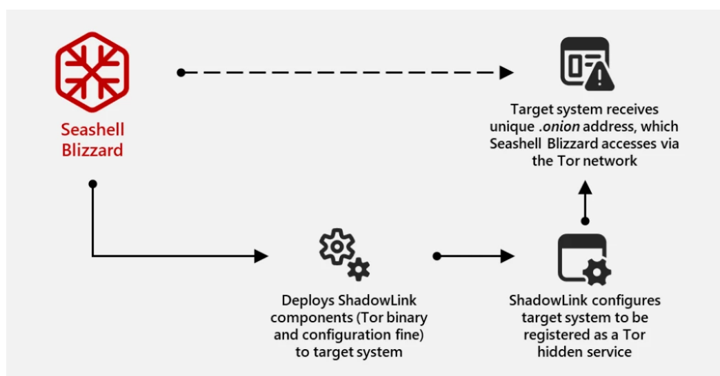
Figure 4. How ShadowLink avoids discovery
