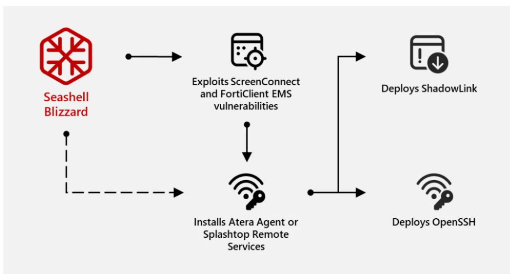
Figure 3. Use of ScreenConnect to install Atera Agent
