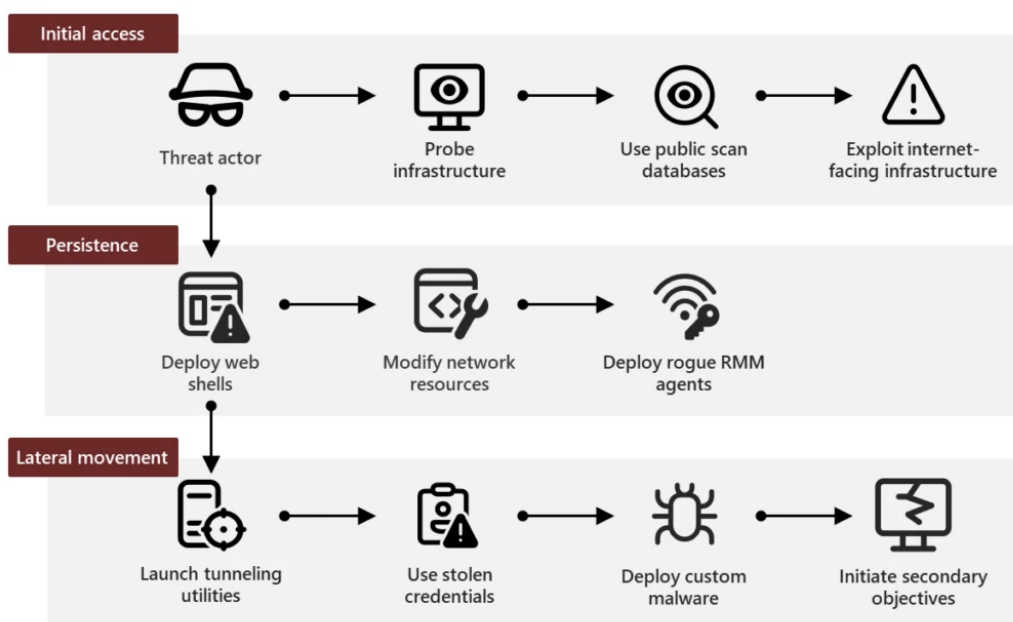
Figure 2. Seashell Blizzard initial access subgroup operational lifecycle
