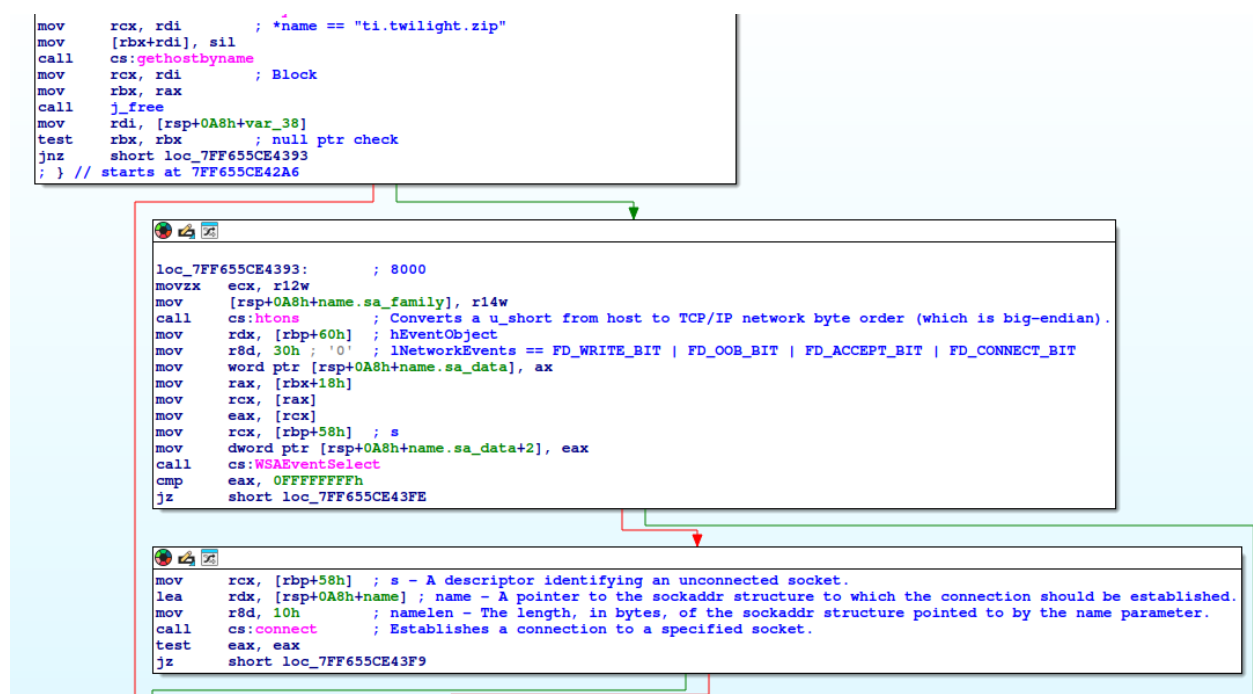
Figure 4 - Resolve C2 and connect
