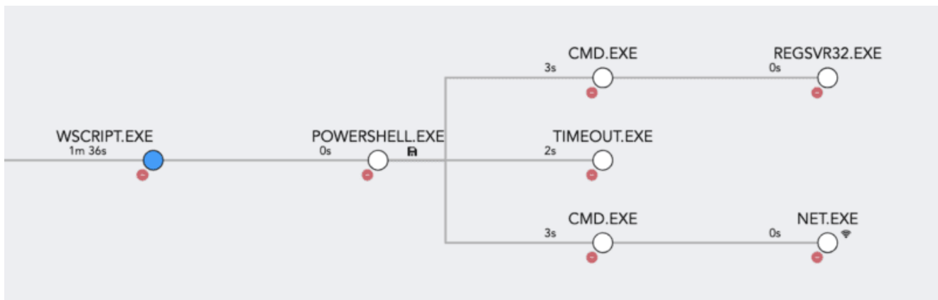
Logpoint Process Tree
