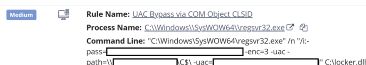
Figure 6: Ransomware Deployment Alerts
