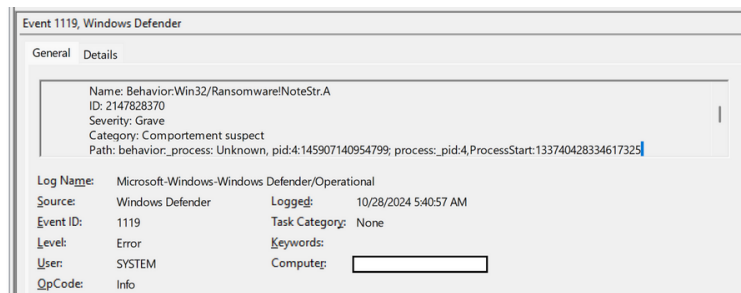
Figure 7: Windows Defender Error Message
