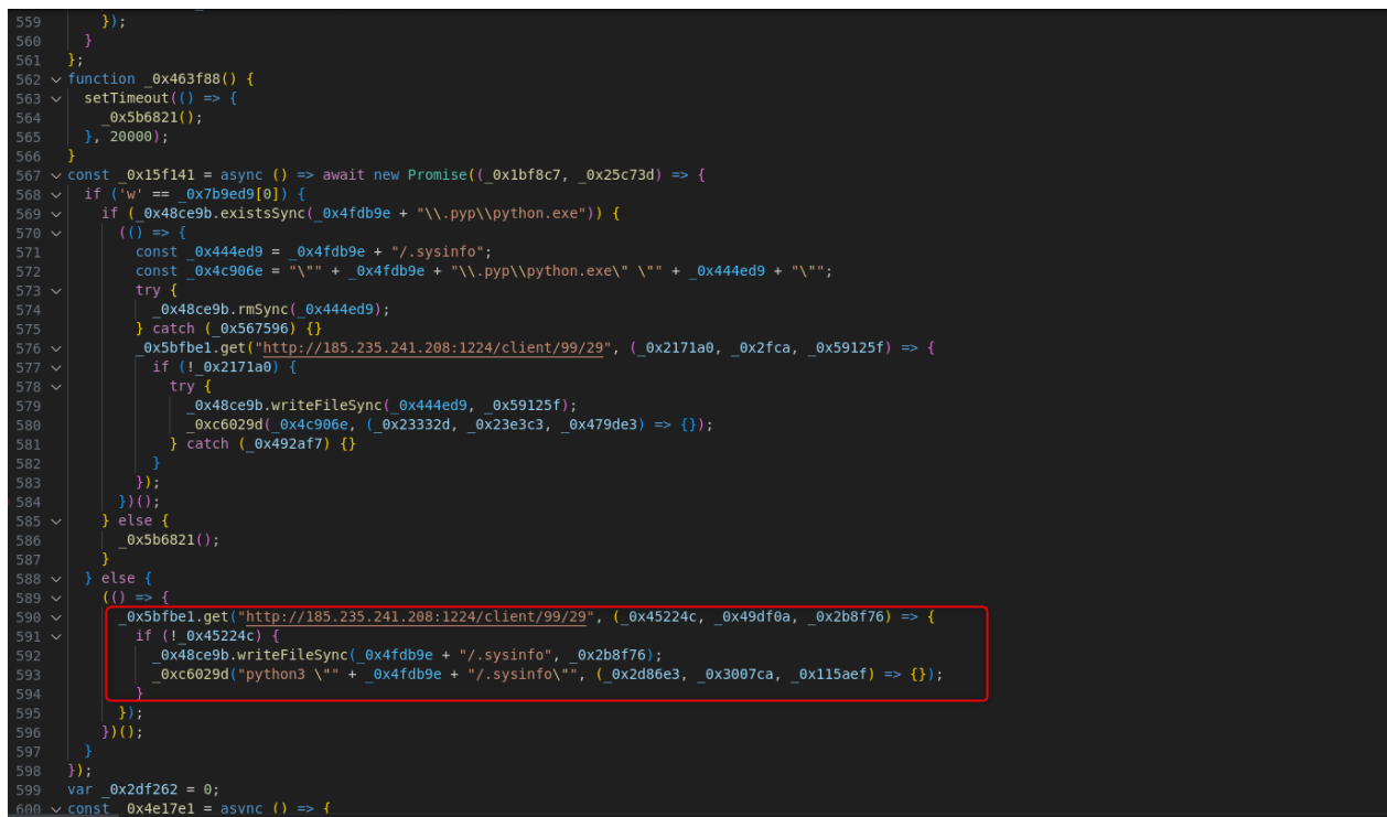
Figure 6 Initial BeaverTail Python Script that Fetches InvisibleFerret.
