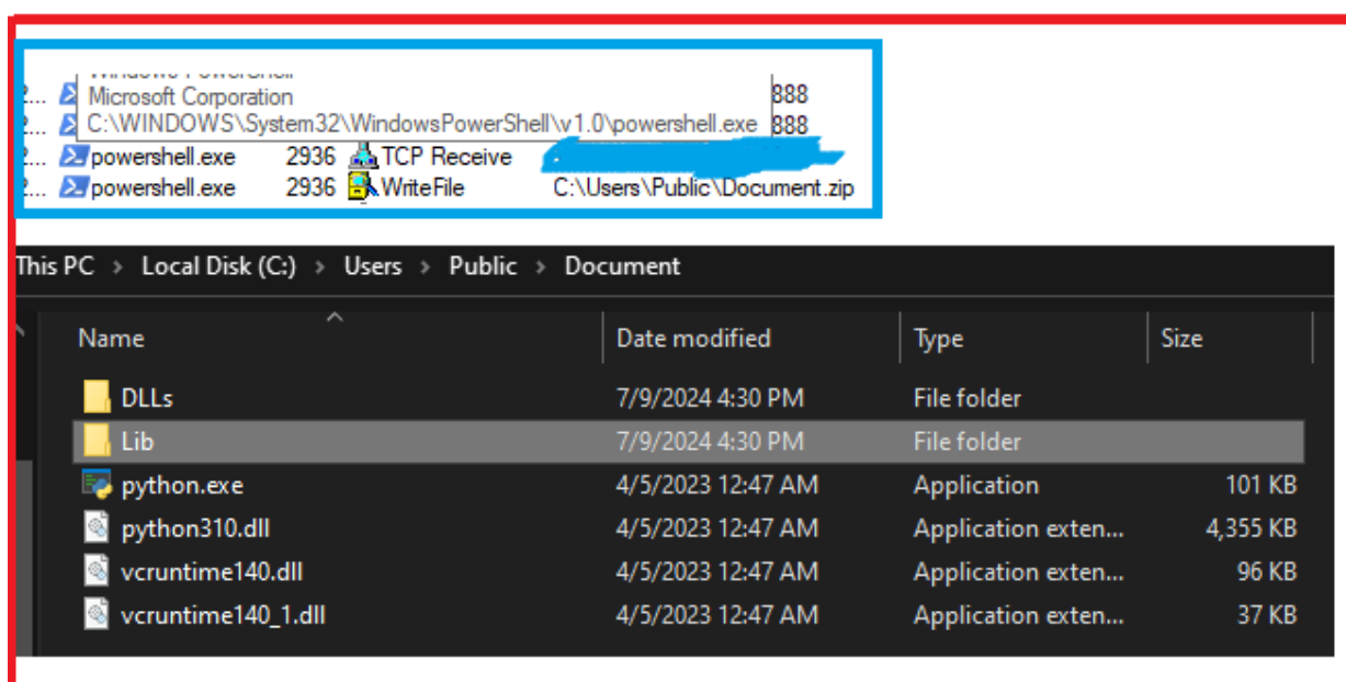
Fig.7: Downloaded contents of Document.zip in “C:\Users\Public”
