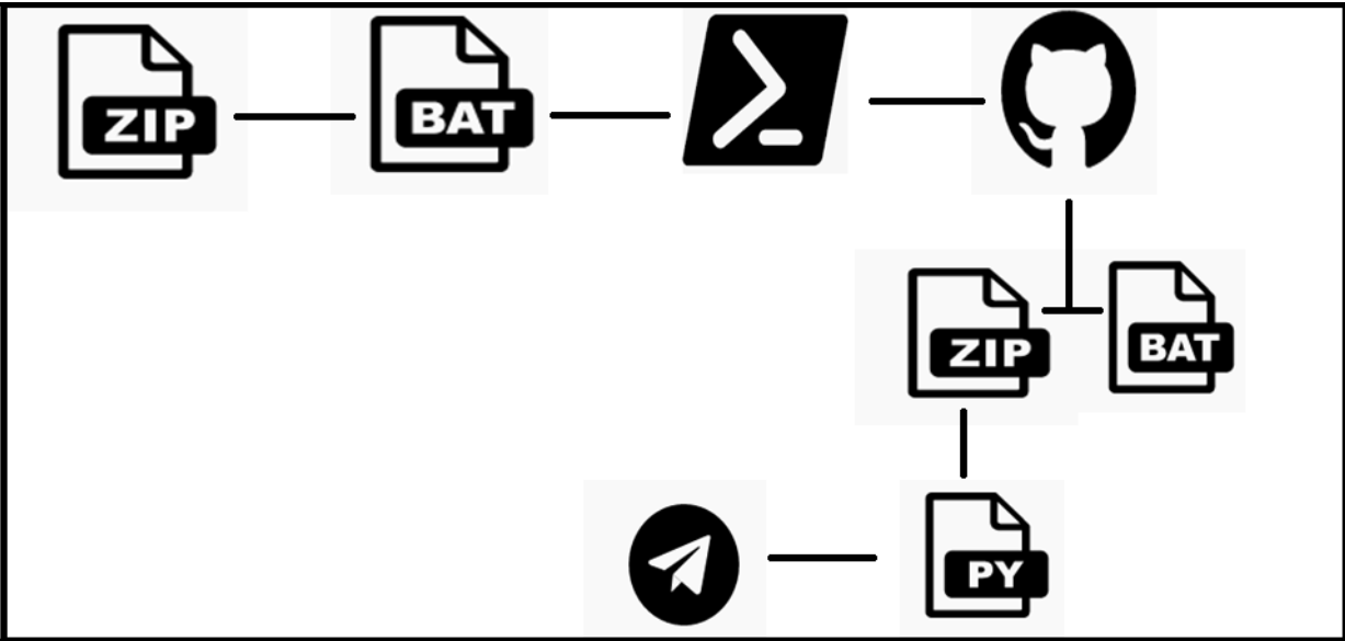
Fig.2: Flow of its execution
