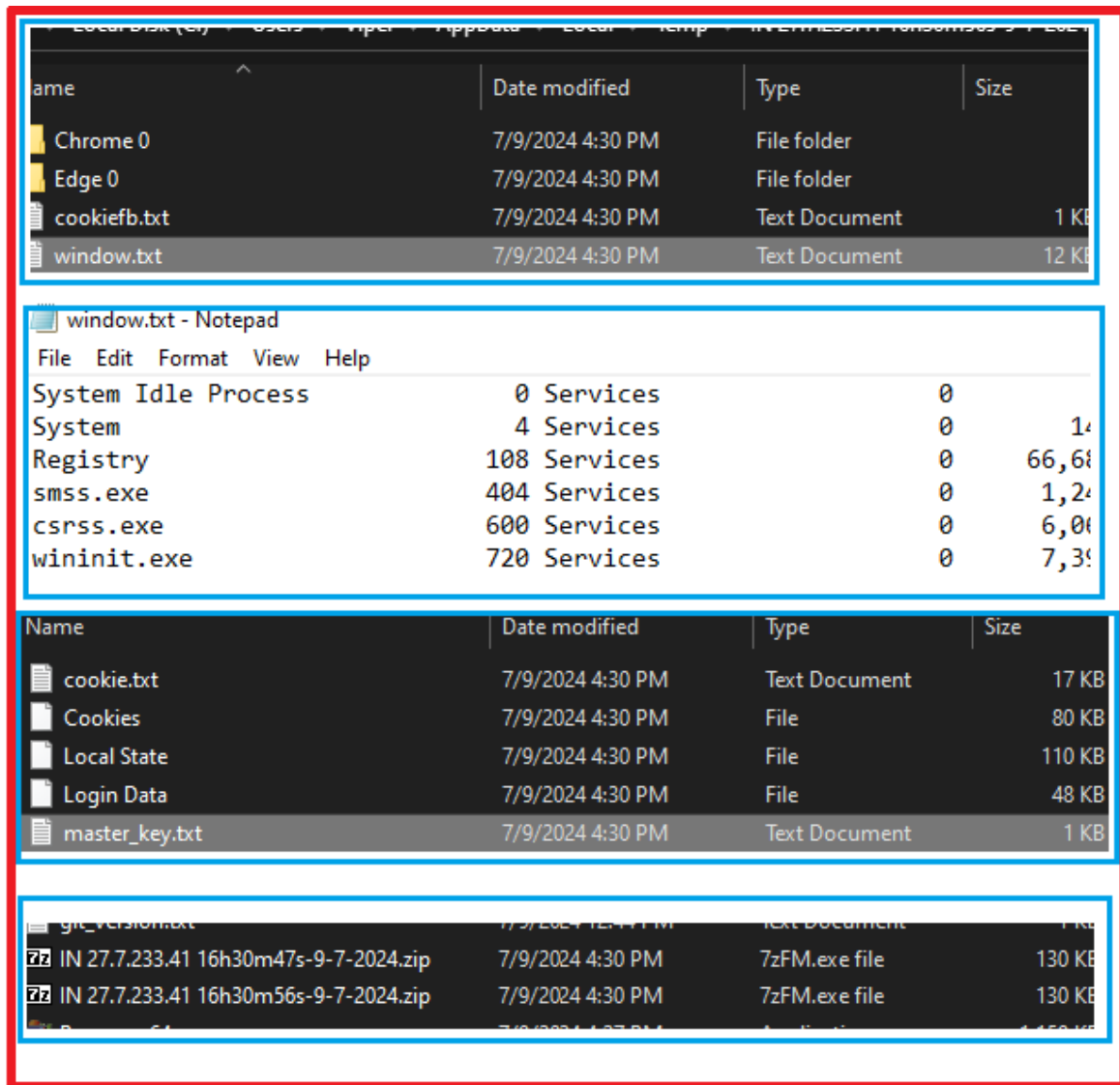
Fig.16: Collected data
