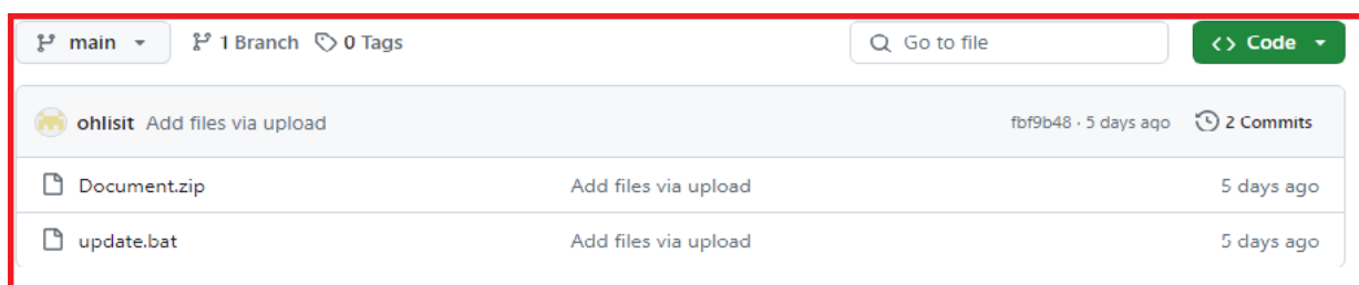
Fig.8: GitHub Repository
