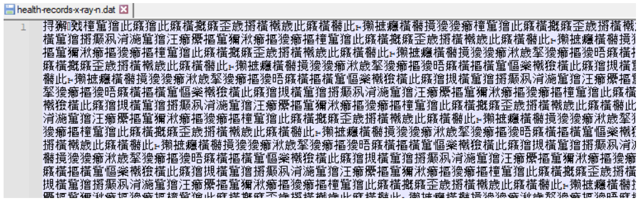
Fig.3: Batch file in notepad++ with “FF FE”
