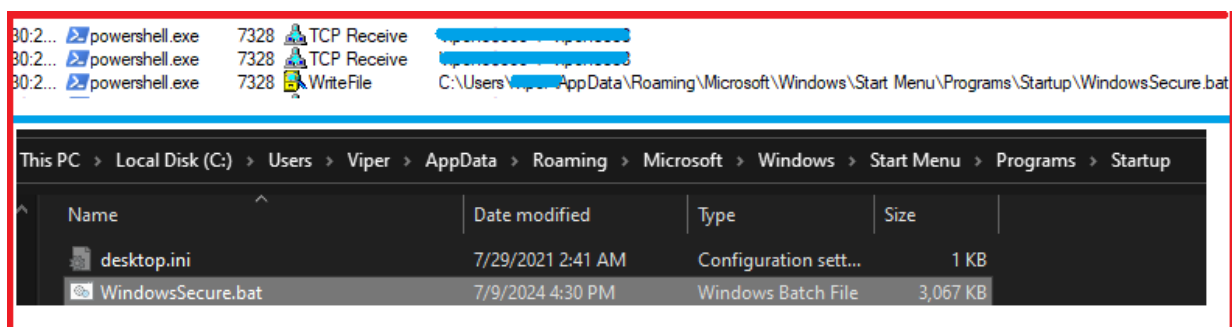
Fig.6: Writing WindowsSecure.bat in the Startup folder
