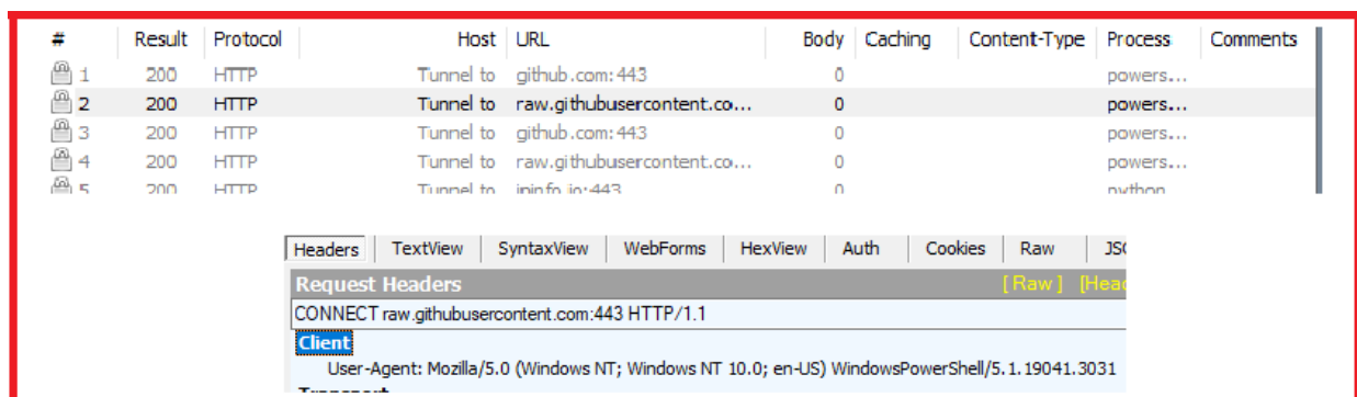
Fig.5: Connection of PowerShell to GitHub
