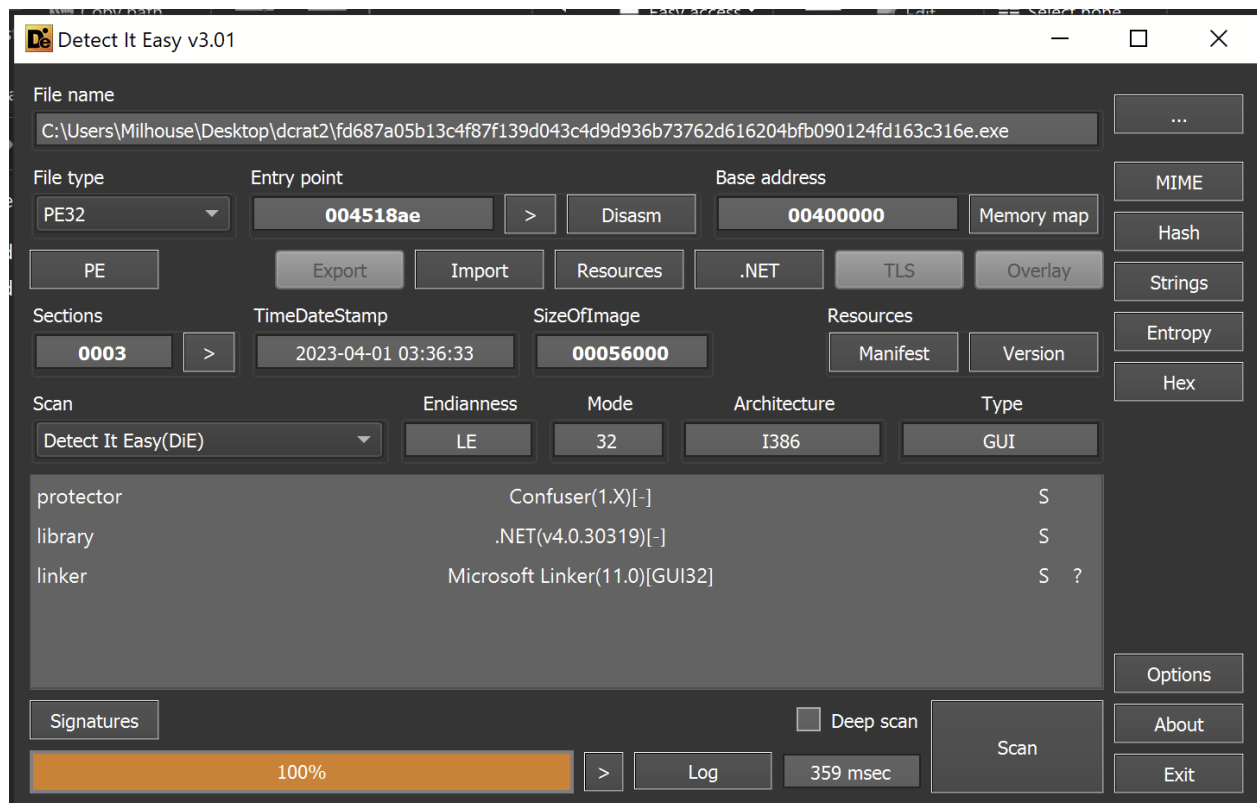
Initial analysis using Detect-it-easy
