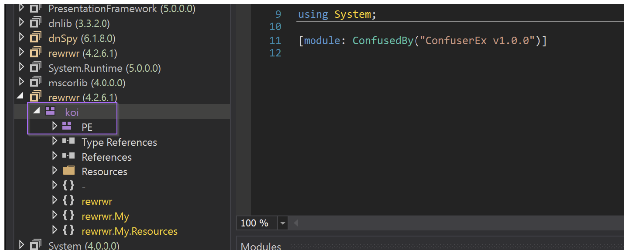
File Overview with Dnspy
