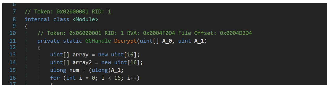
Using Dnspy to locate and view the Decryption function
