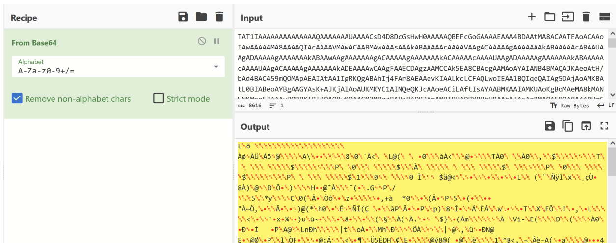
Attempting to Decode Base64 Using Cyberchef - Initially fails due to additional obfuscation
