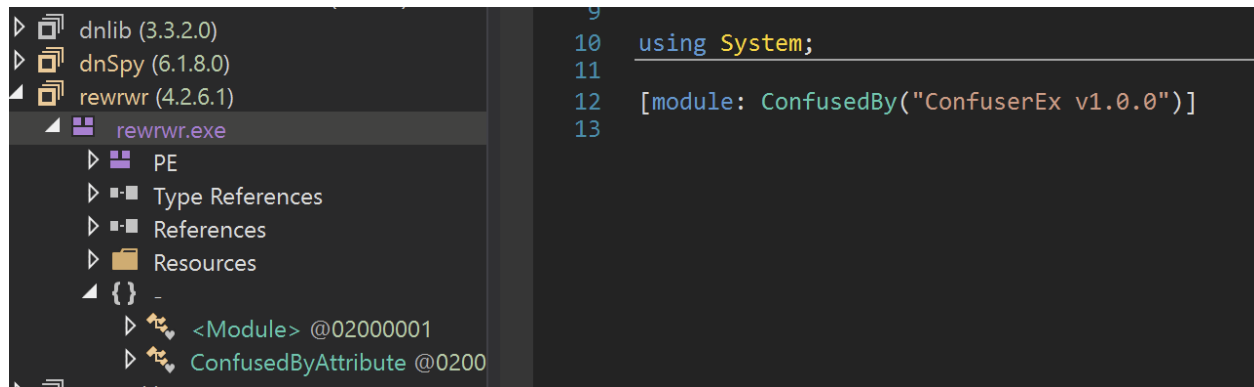
Dnspy overview of the initial file
