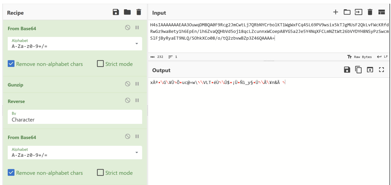
Cyberchef - Additional failures when decoding strings
