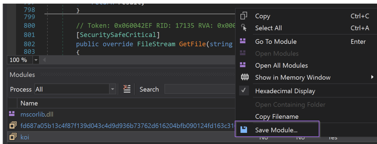
Dnspy Option for Saving a Loaded Module
