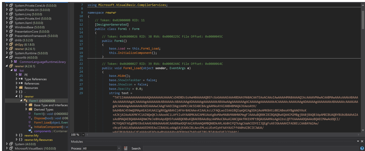
Example of Entry Point Containing Obfuscated Data
