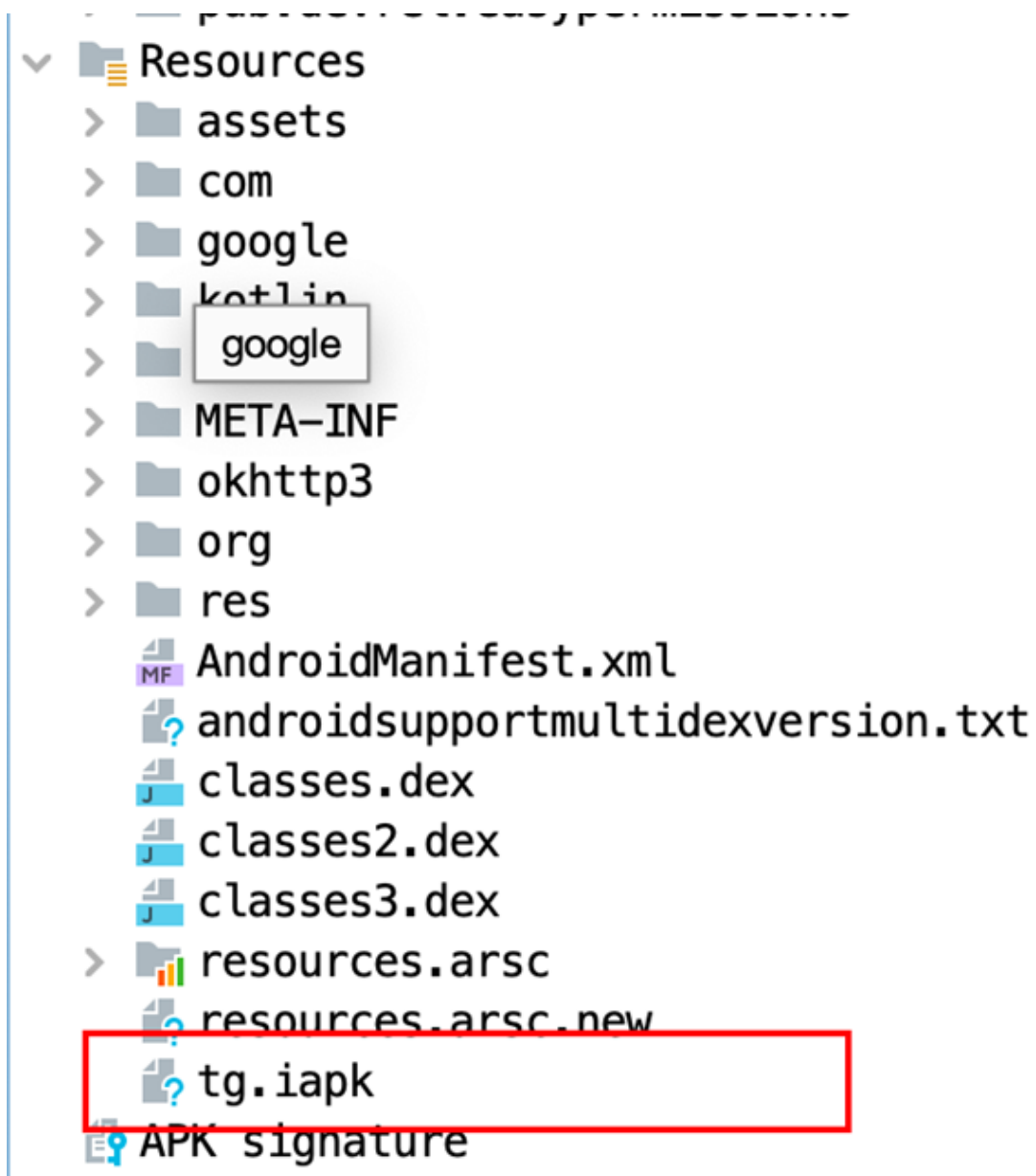
Figure 5. APK structure and the payload
