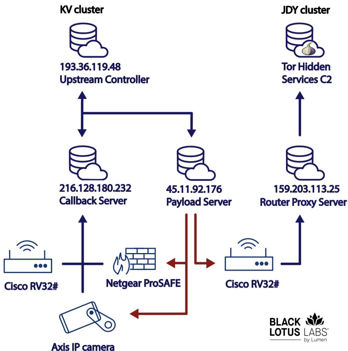
Figure 1: the KV-botnet logical network map, December 2023
