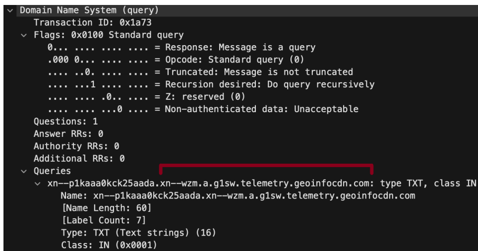
Figure 9. Sample DNS query.
