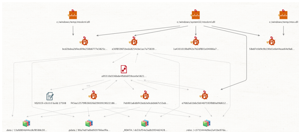
Figure 2. Graph of static features relation across samples.
