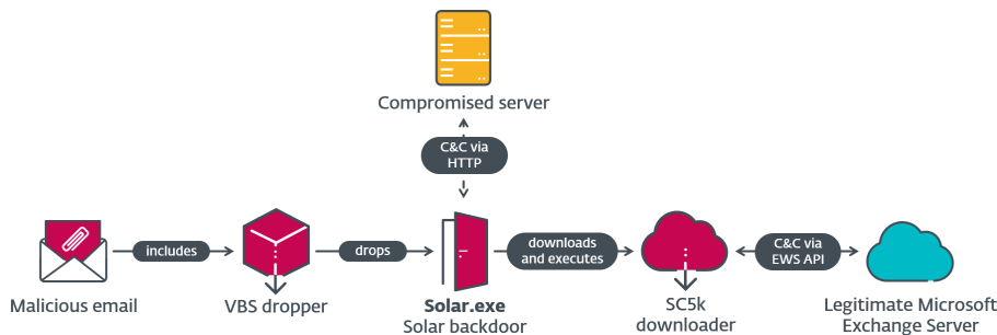
Figure 1. Overview of OilRig's Outer Space compromise chain
