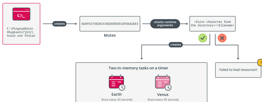
Figure 5. Initial execution flow of Solar
