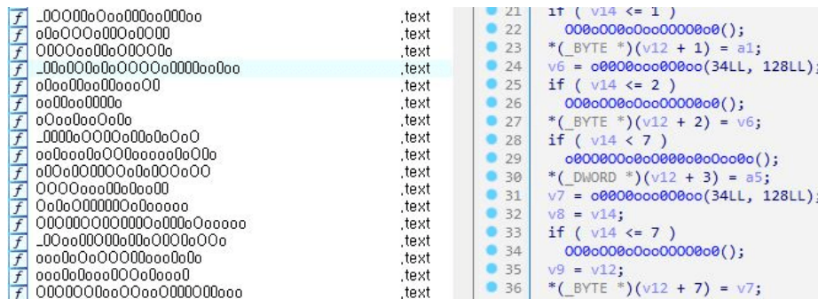
Figure 14. Obfuscated function name
