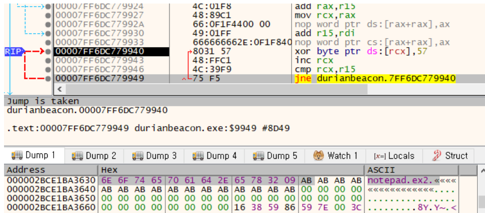
Figure 20. Rust version of DurianBeacon supporting XOR encryption
