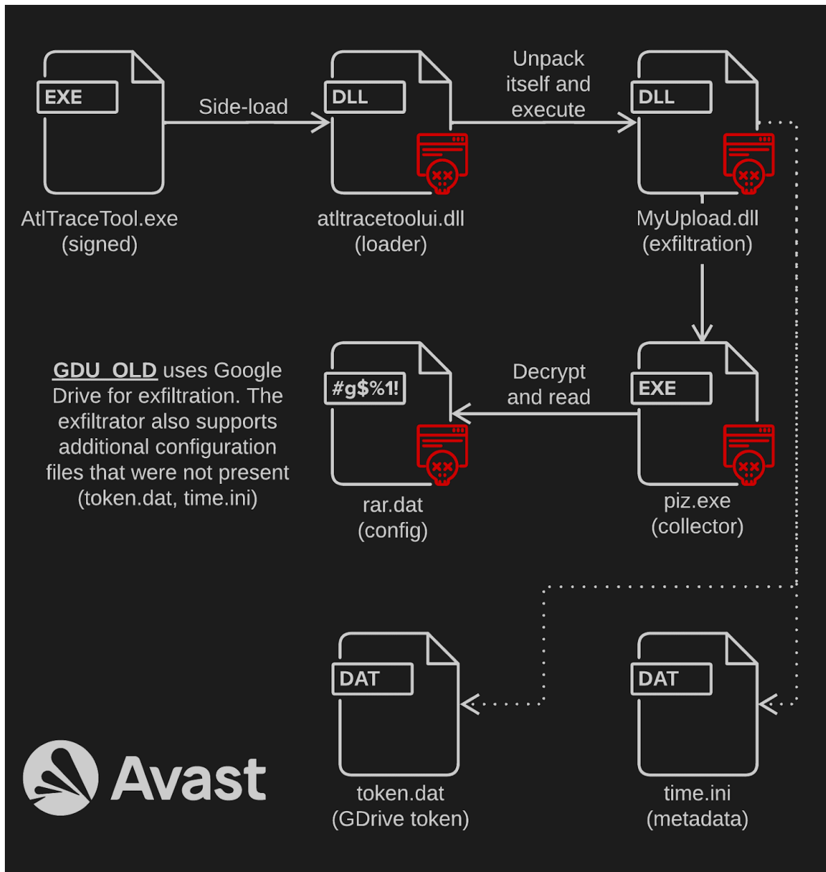
Archive GDU_OLD that uses its own collector piz.exe to collect potentially interesting files before the exfiltration.
