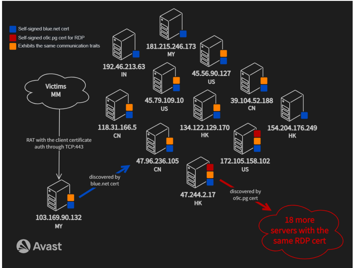
Overview on the servers with ties to JSX RAT C&C.
