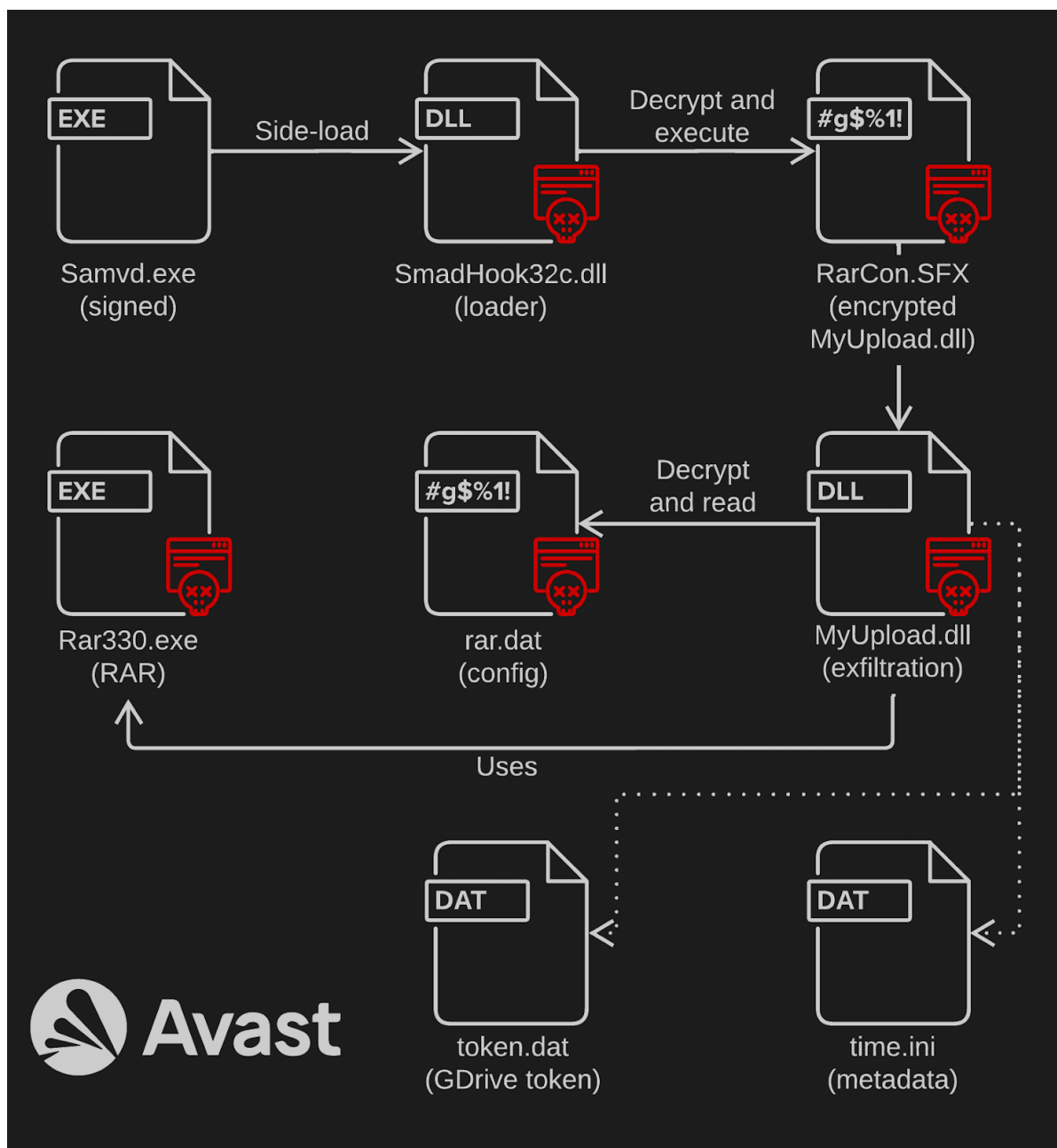
An archive GDU that contains a version relying on RAR instead of piz.exe for data collection.
