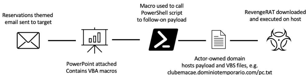
Figure 5: 2020 attack path example
