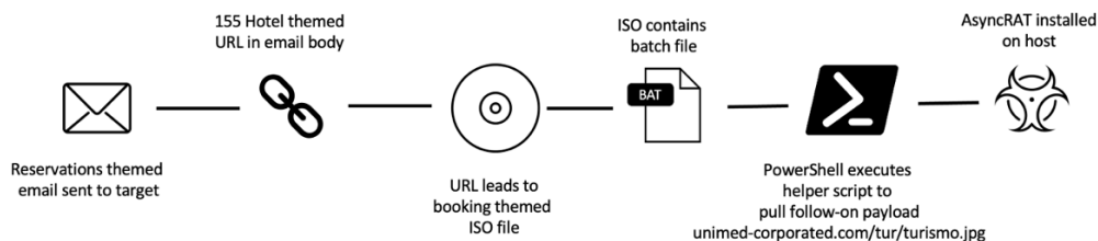
Figure 9: 2022 campaign example chain.
