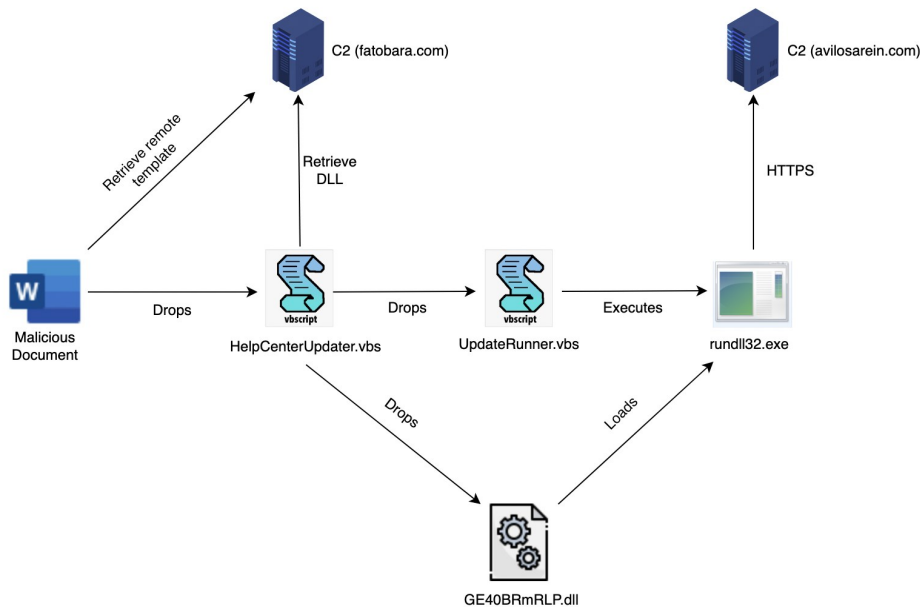
The attack chain for the Saudi Aramco-themed APT campaign
