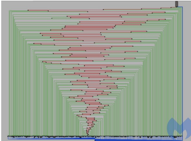
Control Flow Flattening used by the malware
