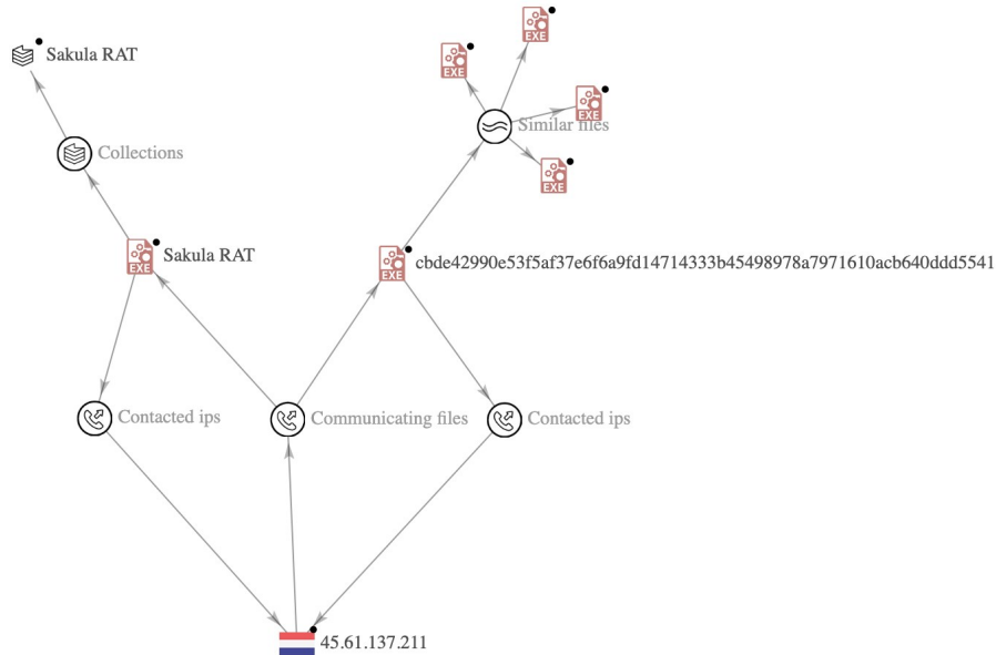
Infrastructure overlap between Sakula RAT and the malware analyzed in this article
