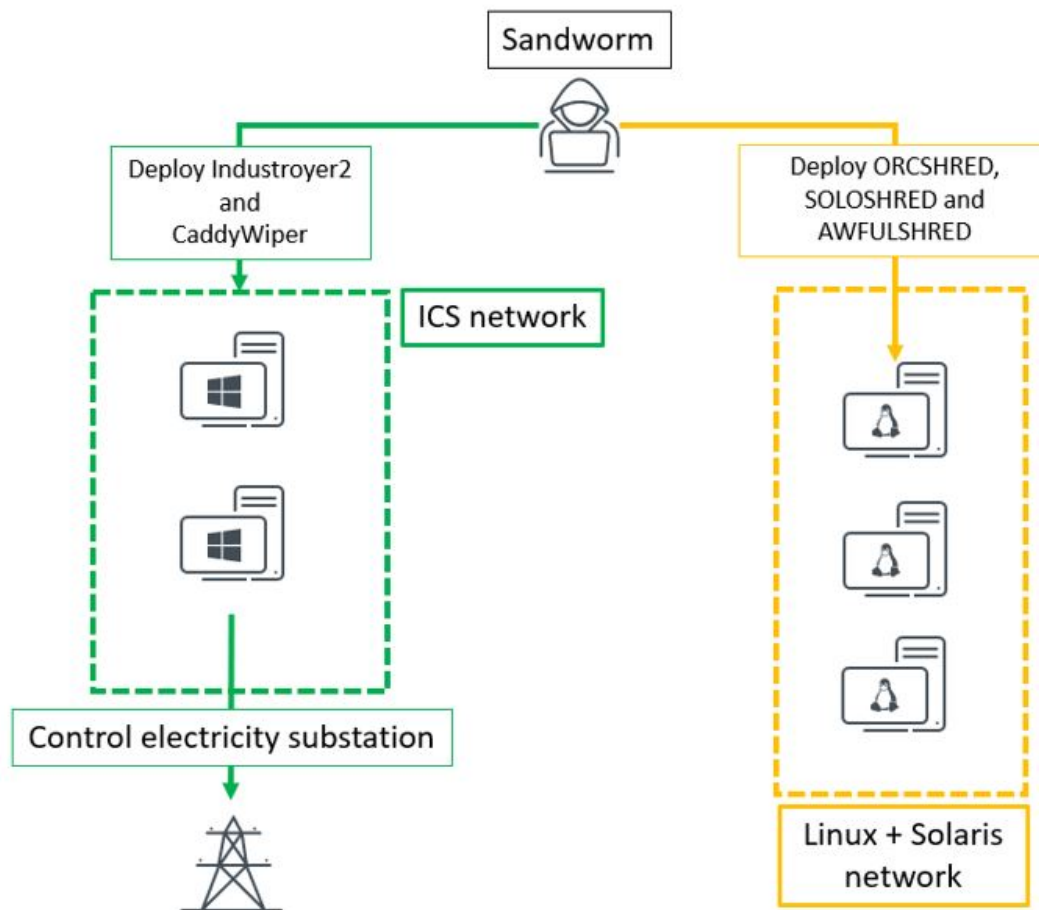
Figure 1. Overview of the malware deployed in the attack
