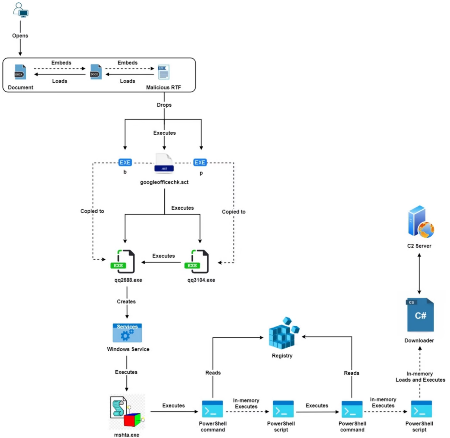
Figure 1: Attack chain
