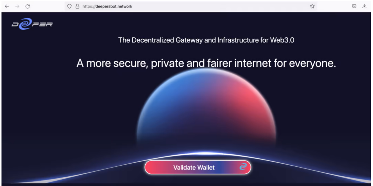
Figure 9: Phishing website
