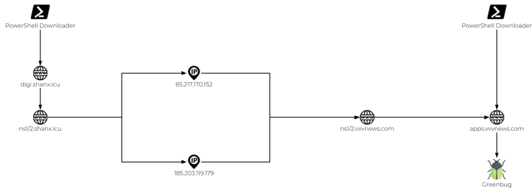
Figure 2. PowerShell and infrastructure overlaps
