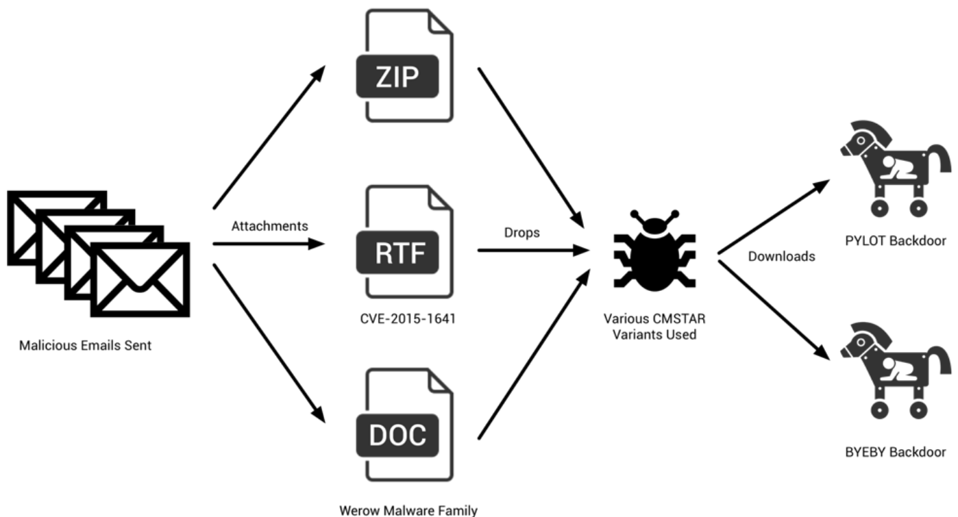
Figure 1 Diagram of the attack sequence
