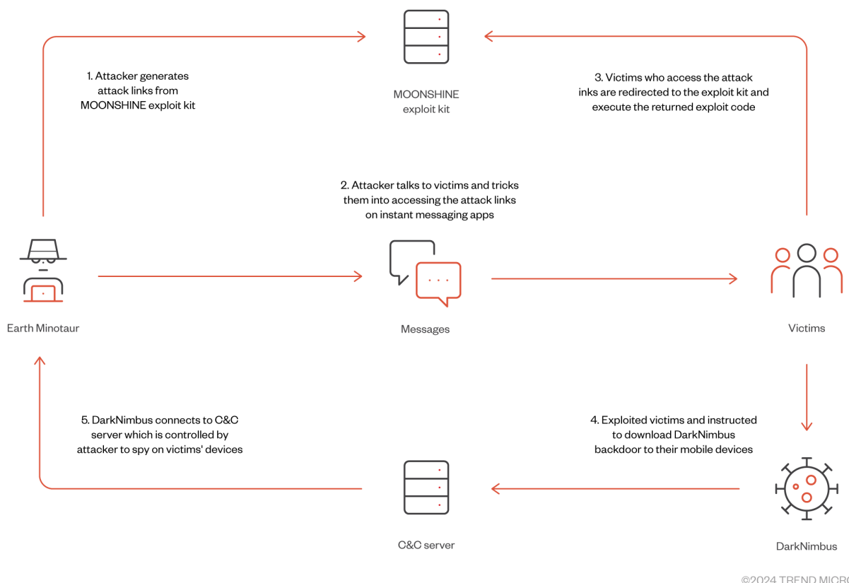
Figure 1. Attack chain of Earth Minotaur
