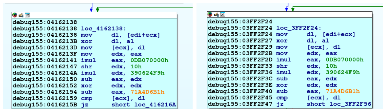
Figure 10. Shadowpad string encryption algorithm for sample with similar C&C (left) versus ESET's sample (right)
