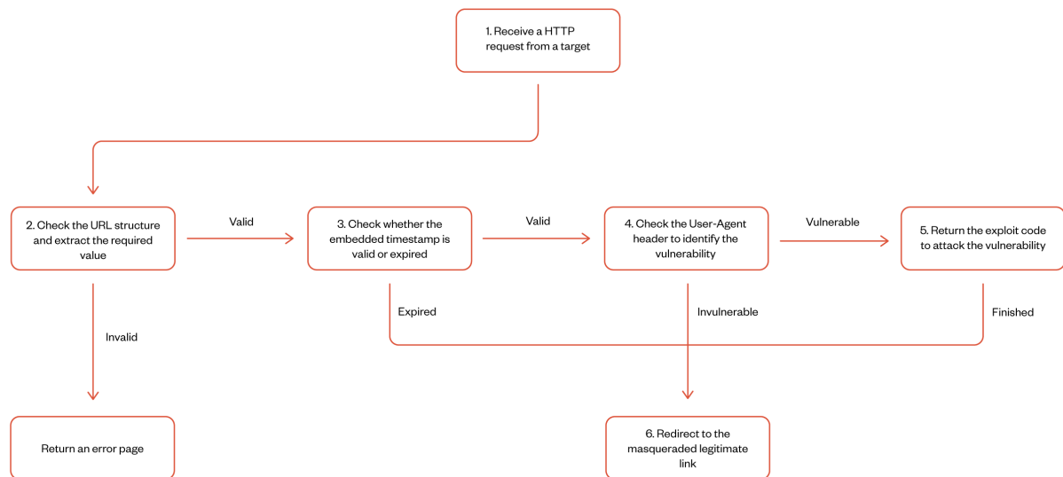
Figure 3. Validation flow of the MOONSHINE exploit kit
